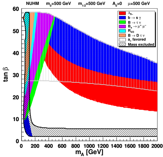
Figure 2: Constraints in NUHM ( m_A - \tan \beta ) parameter plane. For the description of the various coloured zones see the text. The contours are superimposed in the order given in the legend.
