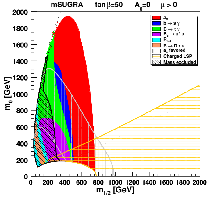
Figure 1: Constraints in CMSSM ( m_{1/2} - m_0 ) parameter plane. For the description of the various coloured zones see the text. The contours are superimposed in the order given in the legend.
