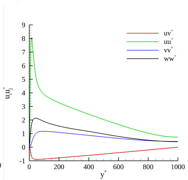
Figure 4: Velocity covariances in viscous units
