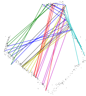
(b) Map-to-Map Reliability : Matching was attempted between every pair of non-consecutive submaps. Shown here are the eight false positives sets with five correspondences. The true positive was not found in this run since only two features were shared between the first and final submaps (See Fig. 3).
