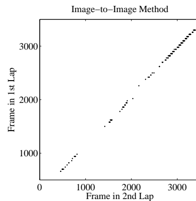
(d) Image-To-Image Reliability : Correspondences were found between every frame in a second lap and every 40th frame in the first lap. A threshold was chosen to remove all false positives. At this threshold, the system was successful in 8% of attempts. To see the effect of the threshold on performance see Fig. 5. Gaps are in regions of the world with lots of foliage (where the image-to-map method also struggles).
