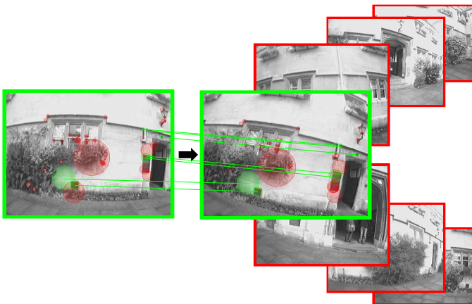
(c) Image-To-Image : Loop closure detected using the method of Cummins et al. [4]. The system detects visual words in each image and the cooccurrence of these words is used to calculate the probability of loop closure. The system finds a high probability that the most recent image matches one seen earlier in the sequence. Visual words are detected in the two images are indicated in green if they match in the other image. Note that interest point geometry is not considered.
