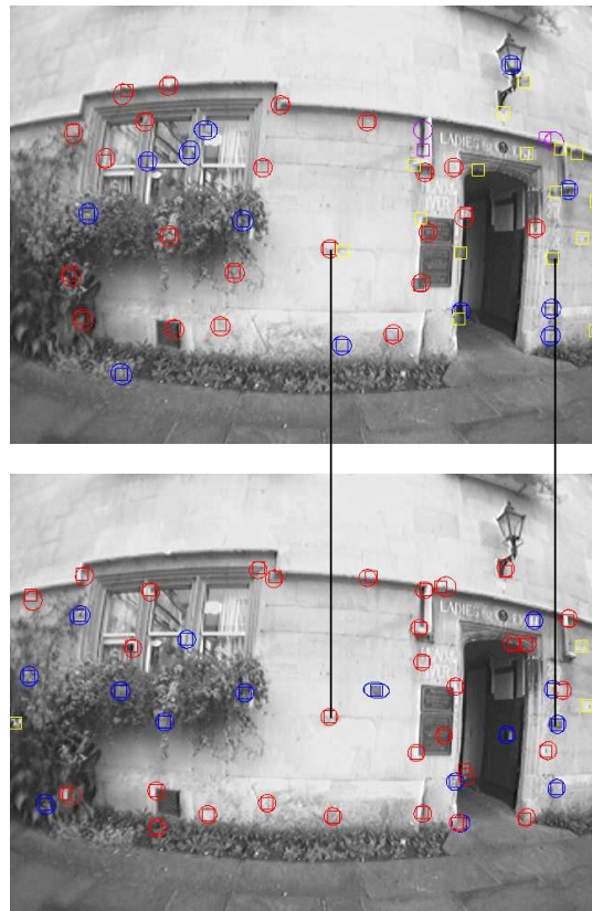
Fig. 3. During the overlap in the sequence, the system tracks the camera in two submaps. The colours indicate if an observation was successful (red), unsuccessful (blue), rejected by JCB (purple), or not attempted, (yellow). Only two of the features are actually common to both submaps. This makes it impossible for the map-to-map method to detect the loop close.
