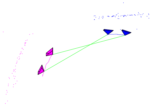
Fig. 2. While tracking in the twelfth map (left), the system localises in the first submap (right) using our image-to-map algorithm. The two submaps are merged by first aligning the common trajectories, and then enforcing the constraint that the two sets of corresponding camera poses (linked by green lines) are equal.
