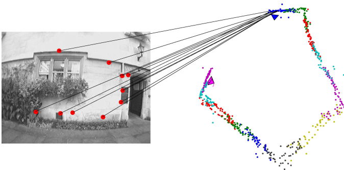
(e) Image-To-Map : Loop closure detected using the method of Williams et al. [13]. While tracking in the last submap, the system finds a camera pose consistent with the features in the first submap. The common trajectory is used to determine the relative rotation translation and scale needed to align the submaps.
