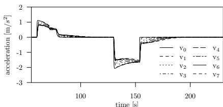
(c) time history of the vehicles acceleration
