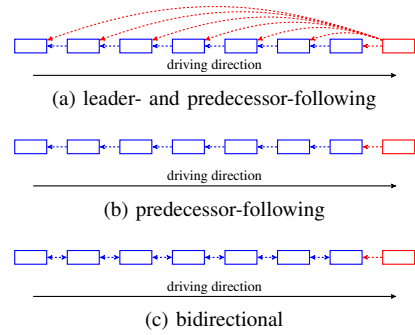
Figure 1. Control topologies selected for the simulations.
