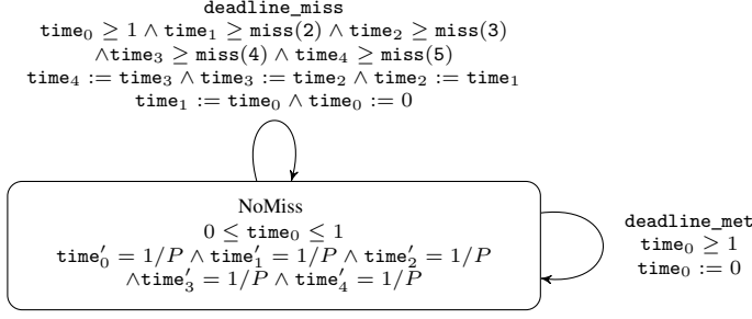
Fig. 3. Scheduler property model based on TWCA as modeled in SpaceEx.
