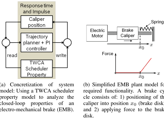
Fig. 4. EMB case study: concrete timing-aware closed-loop analysis and plant functionality
