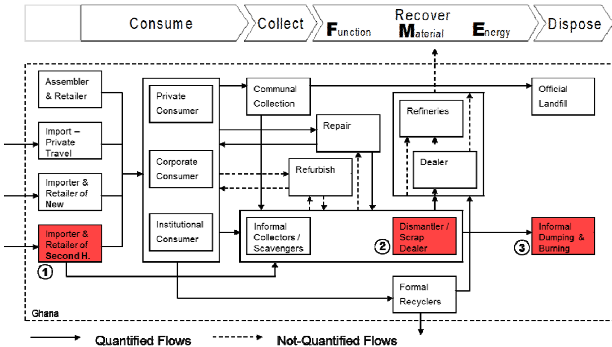
Figure 8.1 Massflow Chart Indicating Hot Spots
