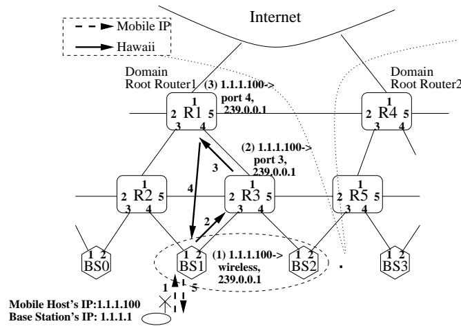
Figure 3: Power-up
