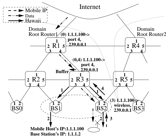
Figure 5: Paging
