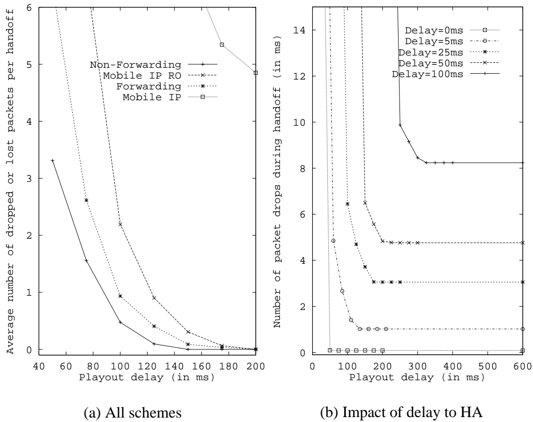
Figure 7: Packet loss during 2-hop handoff
