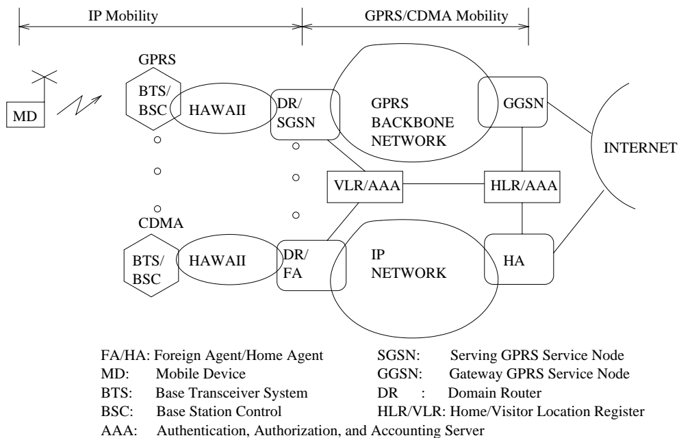
Figure 9: HAWAII in the access network
