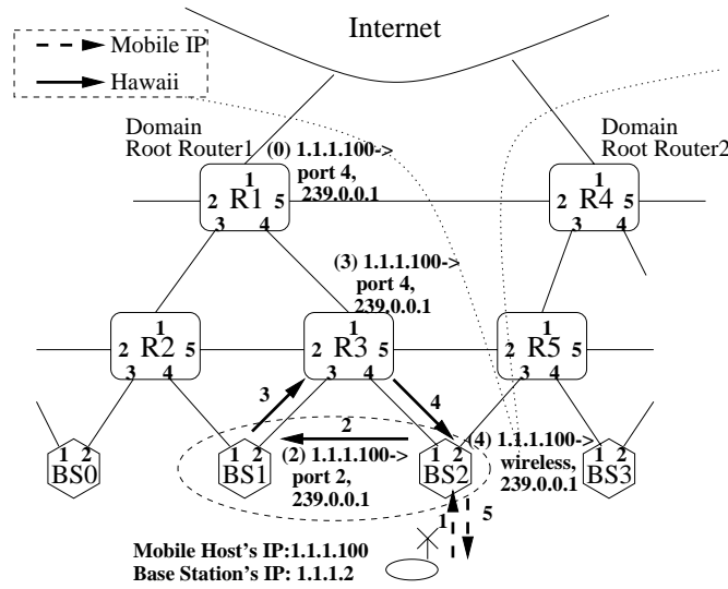
Figure 4: Intra-domain handoff
