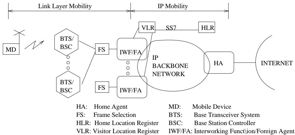
Figure 2: CDMA
