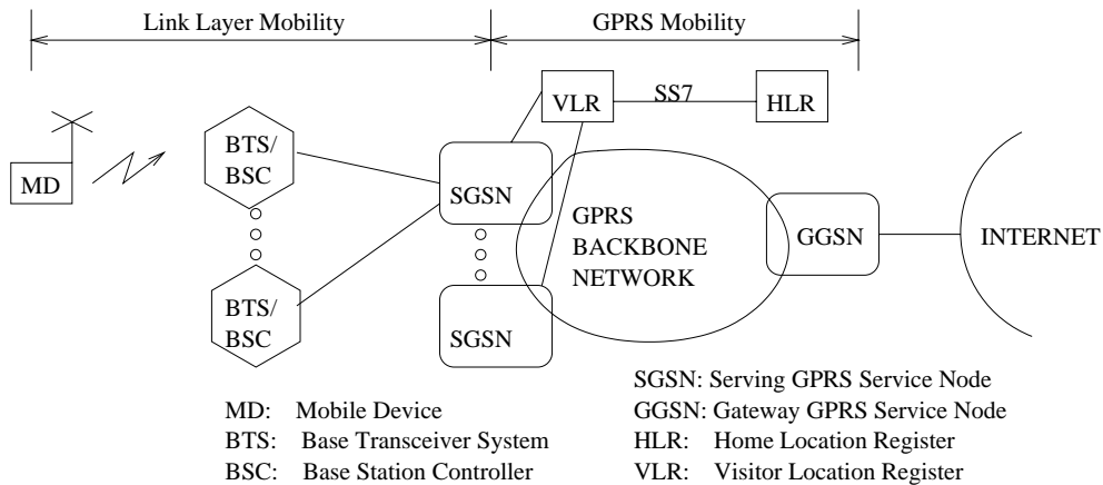
Figure 1: GPRS
