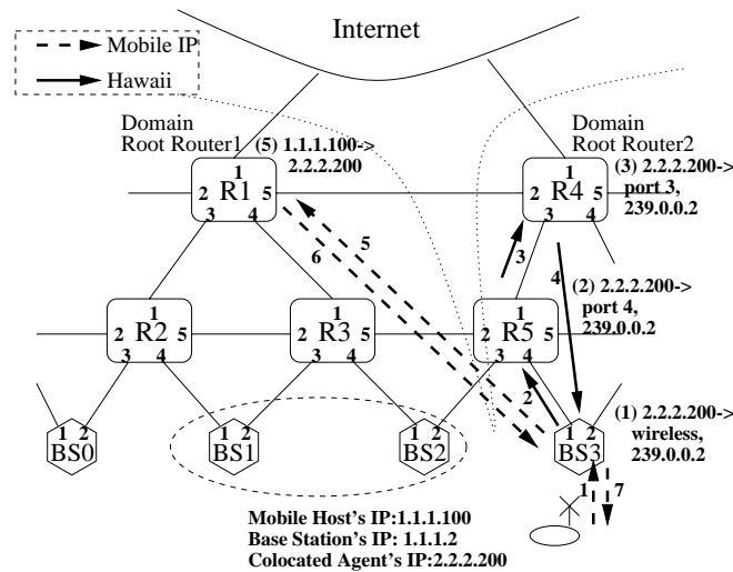
Figure 6: Inter-domain handoff
