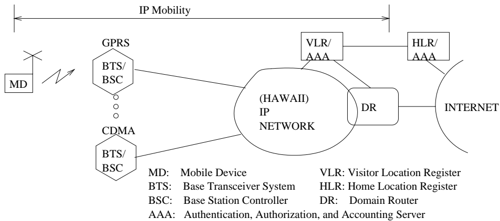
Figure 8: HAWAII-based architecture
