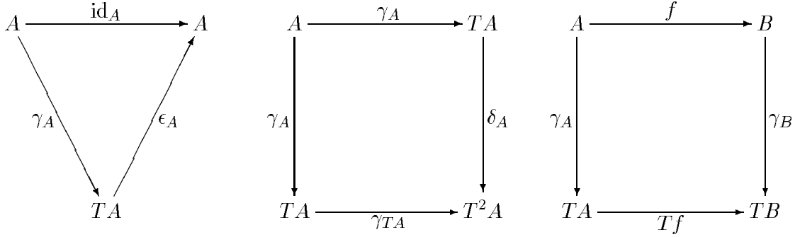
Figure 3: Properties of a computational comonad: these diagrams commute, for all A, B , and all morphisms f : A \rightarrow^{\mathcal{C}} B .
