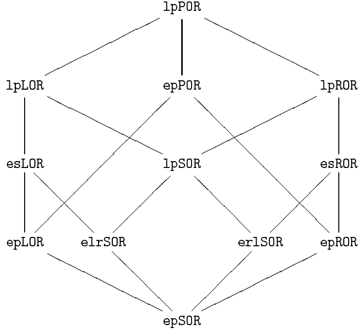
Figure 4: Some algorithms for or-functions, ordered intensionally
