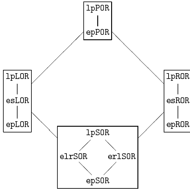
Figure 5: The or-algorithms, quotiented by input-output equivalence
