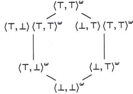
Figure 5. Some paths in T_1(\text{Two} \times \text{Two}) .
