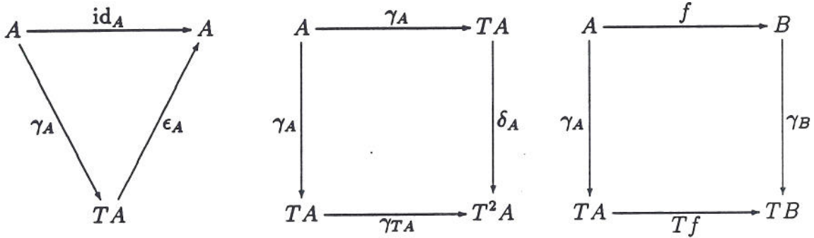
Figure 10. Properties of a computational comonad: these diagrams commute, for all A, B , and all morphisms f : A \rightarrow^{\mathcal{C}} B .
