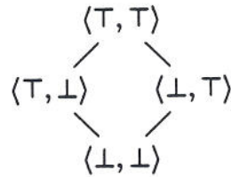
Figure 3. The domain \mathbf{Two} \times \mathbf{Two} .
