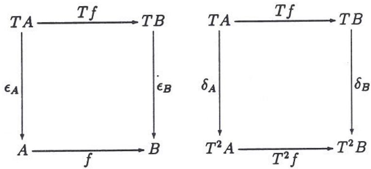
Figure 1. Naturality of \epsilon and \delta in a comonad: these diagrams commute, for all A, B, f : A \rightarrow^c B .
