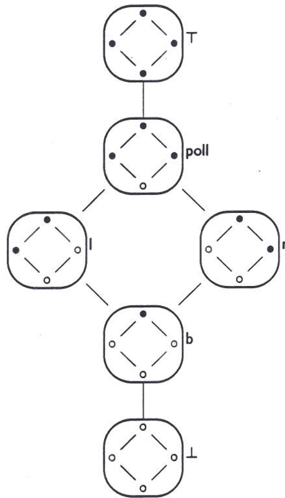
Figure 4. Continuous functions from \mathbf{Two} \times \mathbf{Two} to \mathbf{Two} , ordered pointwise.
