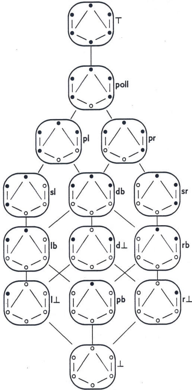
Figure 8. Some T_2 -algorithms from Two \times Two to Two , ordered pointwise.
