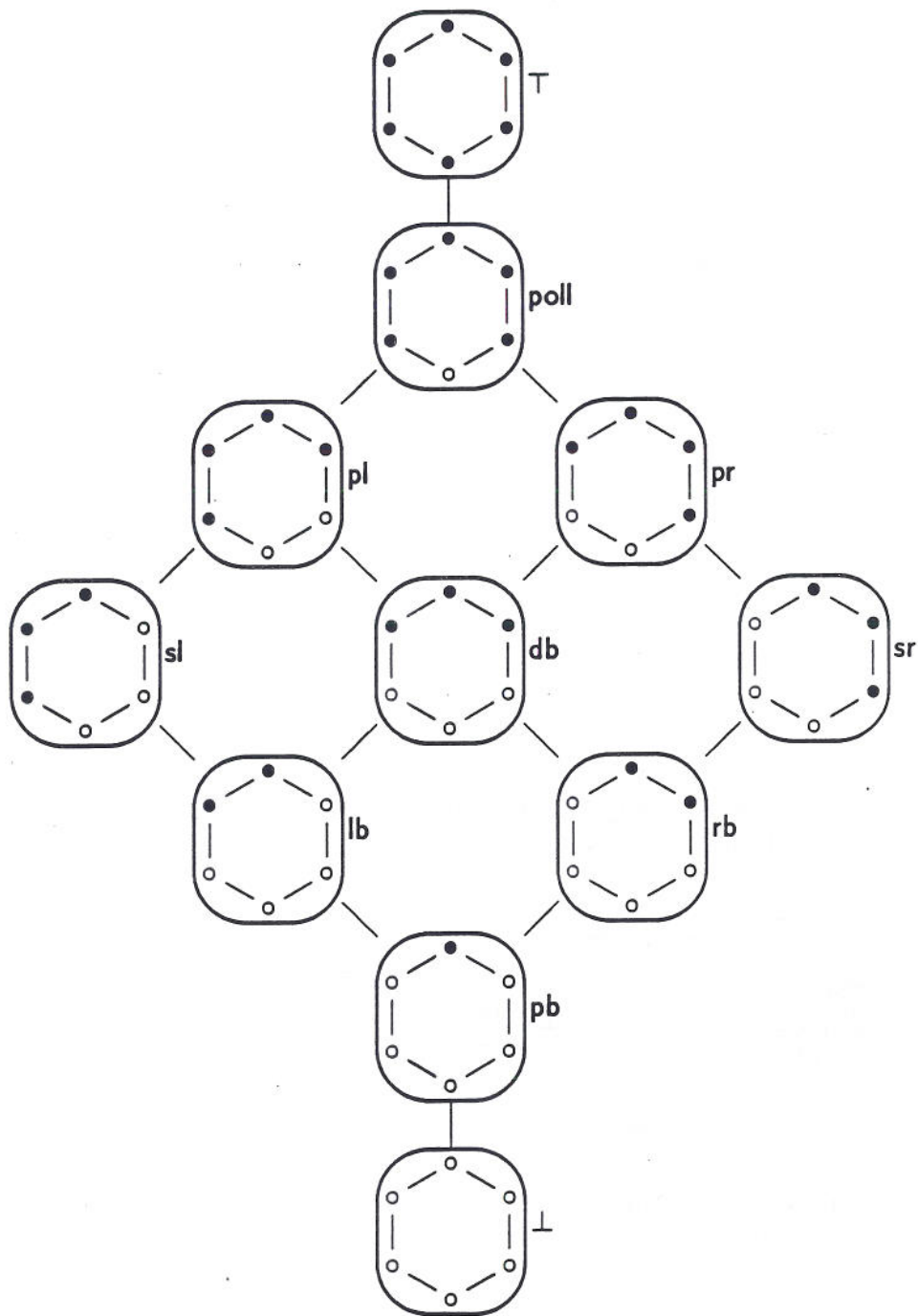
Figure 6. Some T_1 -algorithms from \mathbf{Two} \times \mathbf{Two} to \mathbf{Two} , ordered pointwise.
