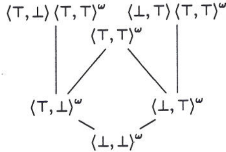
Figure 7. Part of T_2(\text{Two} \times \text{Two}) .
