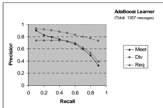
Figure 5 - Precision/Recall of 3 different classes using AdaBoost
