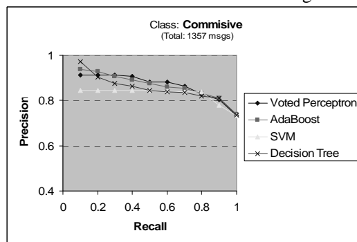
Figure 3 - Precision/Recall for Commissive act
