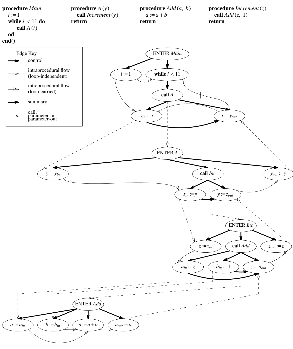
Figure 9: The SDG from figure 8 sliced with respect to the formal-out vertex for parameter z in procedure Increment , together with the system to which it corresponds. Note that this slice correctly excludes the vertex labeled x_{in} := su_{10} in figure 8
