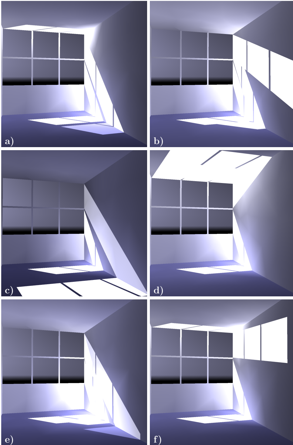
Fig. 7. Sample CFS renderings in a small test room with south facing windows at 10am on March 21st. The bottom 3 window panes are plain glass in all images. The top 3 panes are: a) laser cut panel, b) optical film (interior), c) perforated blind (open), d) Lumitop TM , e) mirrored Venetian blind, and f) Serraglaze TM .
