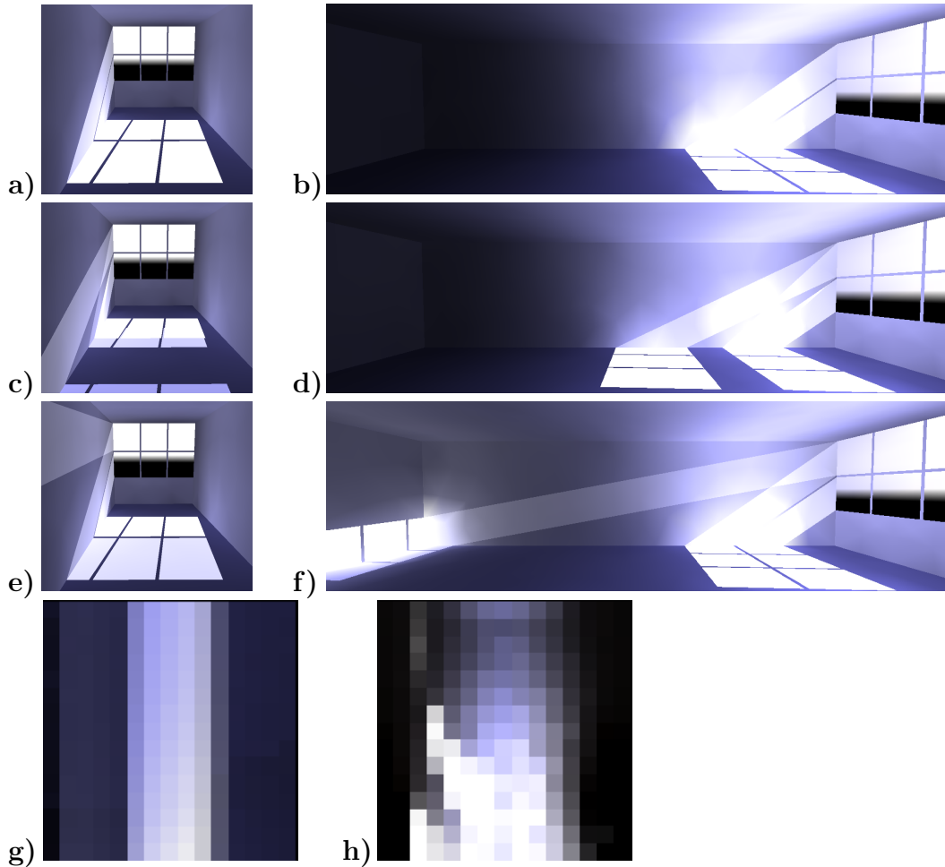
Fig. 4. Initially all six windows in this simple room scene are filled with a&b) simple planar glass. Note how the far back corner of the room is dark. In c&d) we replace the top 3 panes with a prismatic panel having shallow angles and in e&f) we select a more extreme angle for the upper microfacets in these panels, which sends direct light to the far wall to more uniformly illuminate the room. To optimize the material selection for the center point of the floor at a given time and day of the year, we g) vary the two angular parameters of the prismatic material. Fixing the material, we h) vary the time of day and day of year and calculate the illumination on the center point of the floor.
