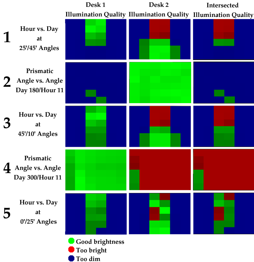
Fig. 10. A multi-stage optimization of the scene shown in Figure 9. The plots are false colored where green indicates levels that fall within the recommended range for reading (200-2000 lux).
