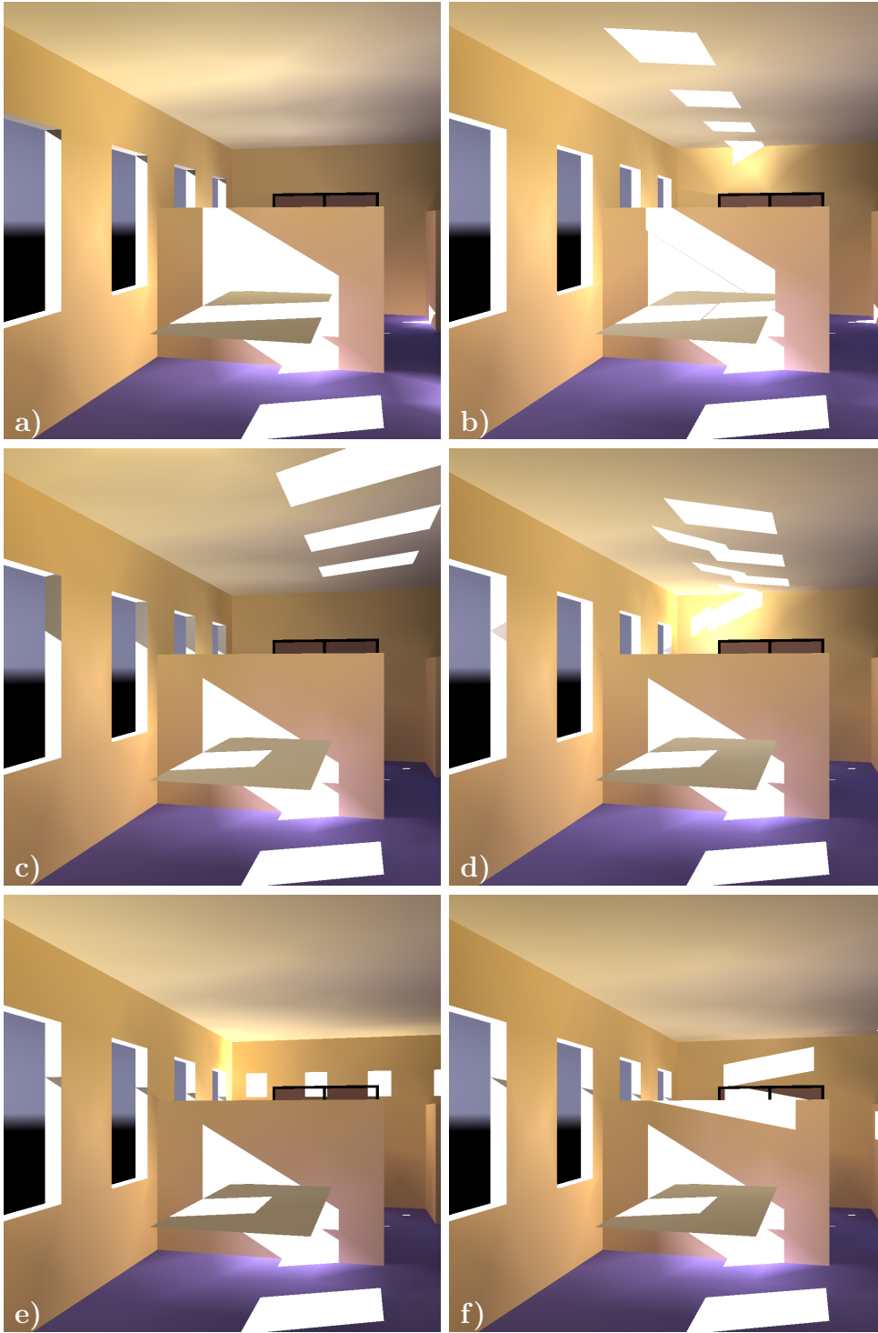
Fig. 8. Sample CFS rendering in a medium-sized office scene with west facing windows at 3:30pm on March 21st. The lower portion of each window is plain glass in all images. The upper portion of each window is a) plain glass, b) laser cut panel, c) mirrored Venetian blind, d) Lumitop TM , e) optical film (interior), and f) Serraglaze TM .
