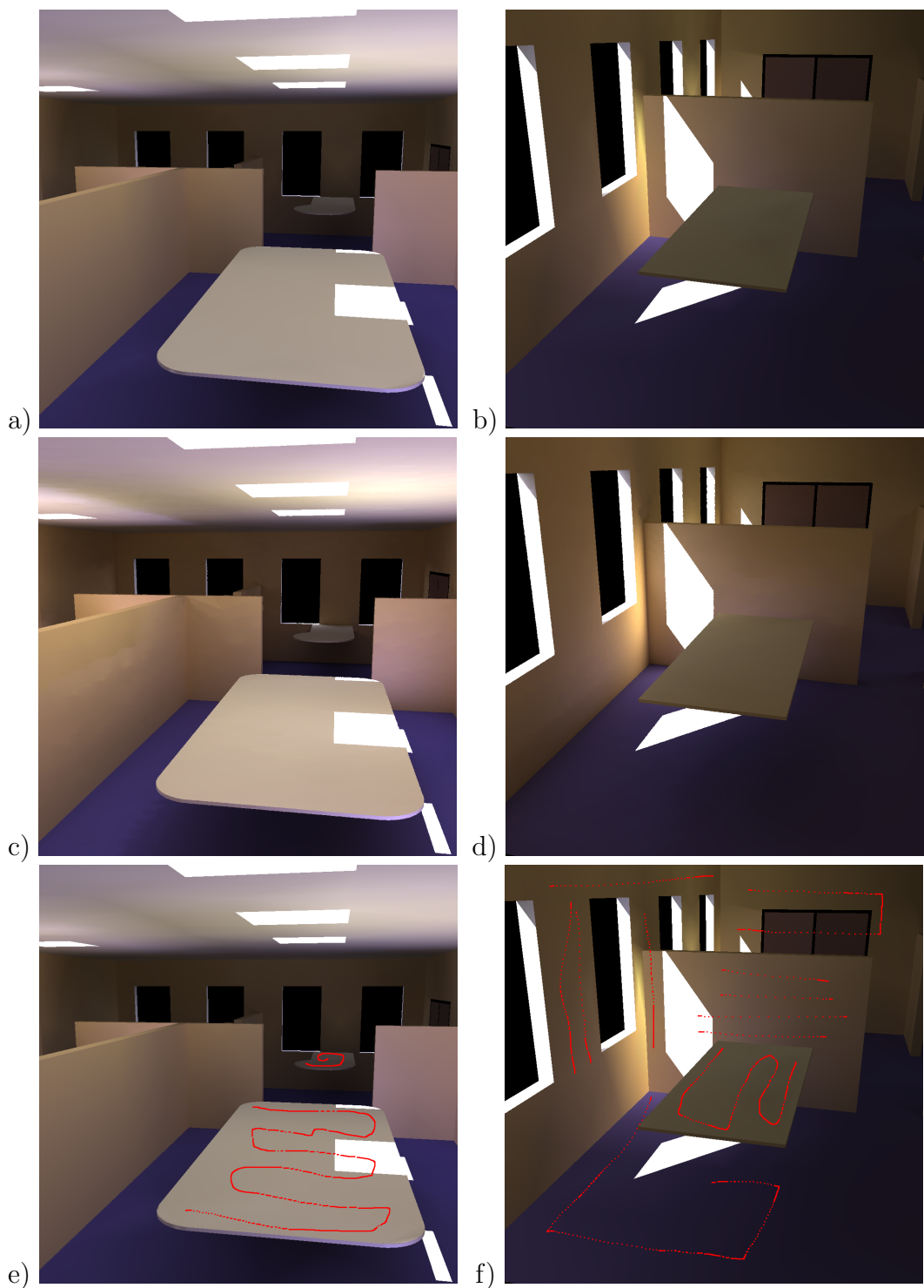
Fig. 14. We performed a quantitative comparison between our system (a & b) and Radiance (c & d). The comparisons were done both over all pixels in the image and on a region of interest marked by the user, (shown in red in images e & f). The numerical results are presented in Table 1.
