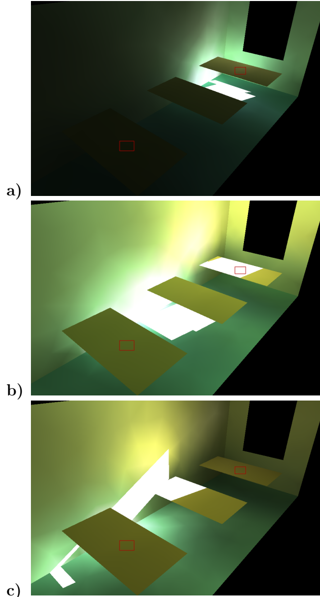
Fig. 9. A simple office scene with a single southern-facing window. The designer uses daylighting optimization to select an appropriate fenestration material to more uniformly illuminate the desks nearest and furthest from the window (outlined with small red squares). The optimization process is shown in Figure 10.
