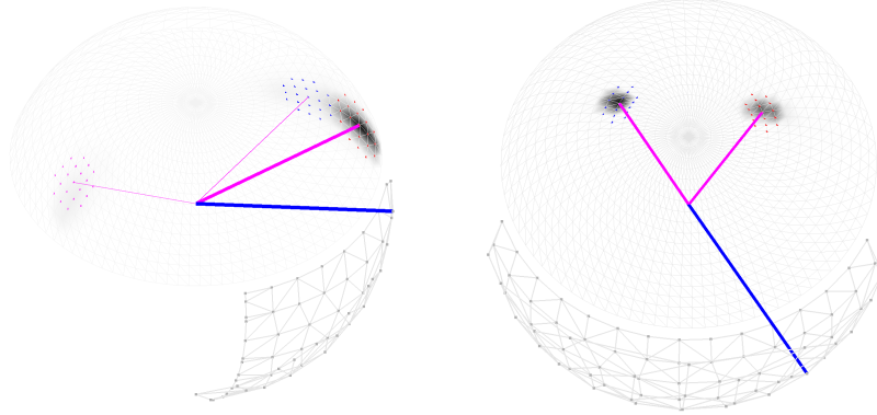
Fig. 6. Plots of the BTDF data for the laser cut panel CFS for two sample incoming light directions (shown in blue). Up to three lobes are fit to the data to model the specular outgoing illuminance (shown with different widths).
