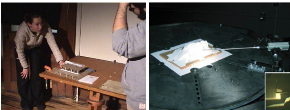
Fig. 1. The depth of direct beam light penetration in a model is easily ascertained with the heliodon . Interior views (right inset) may require endoscopic lenses depending on the model size. The heliodon table rotates along many dimensions relative to a fixed light source (the sun), facilitating exploration.
