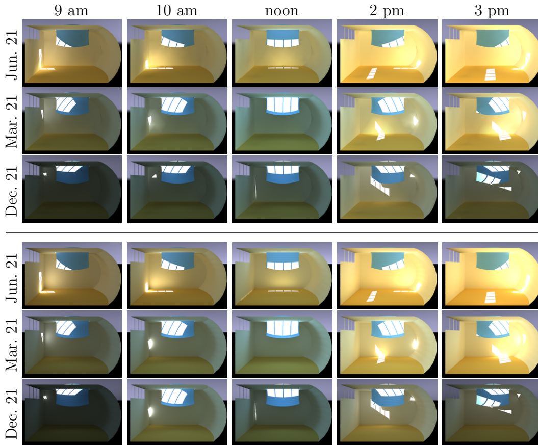
Fig. 12. In designing the interesting curved geometry for the living space in this residential design, the architect redirects the strong overhead noon sunshine from a set of skylights with a curved diffuse blue deflector but allows the warmer late afternoon sun to penetrate deep into the room and wash over the far wall. Our interactive global illumination relighting system allows him to quickly evaluate this geometry for different sun positions and sky conditions. The top 3 rows of images are rendered with our system. The bottom 3 rows are produced by Radiance.
