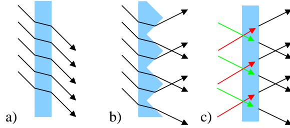
Fig. 3. a) In a flat pane of glass, light rays are refracted, but exit parallel to the input rays. b) Light rays that pass through a prismatic panel are refracted differently and exit in two different directions due to the microfaceting. c) We can reverse engineer the directions of two “fake suns” allowing us to render the specular refraction in real time (Section 3.4).
