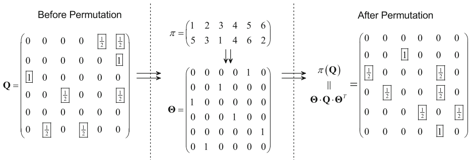
Figure 5 The relationship between permutation \pi and its corresponding permutation matrix \Theta .
