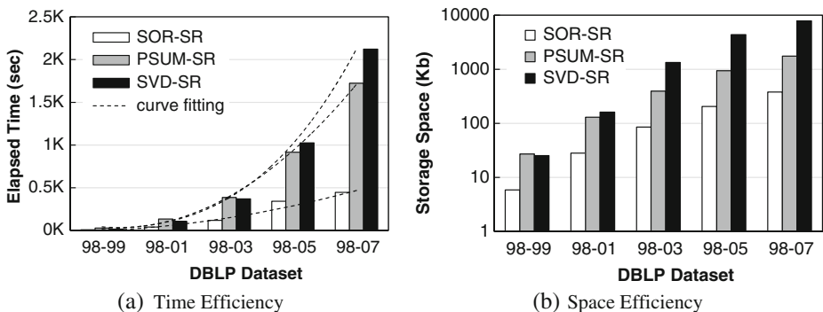
Figure 7 Efficiency and scalability on DBLP datasets.
