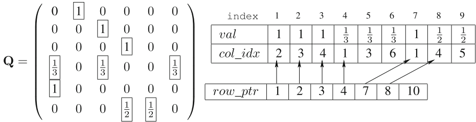
Figure 2 CSR representation of the adjacency matrix \mathbf{Q} .
