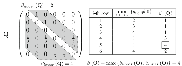
Figure 3 Bandwidth of the adjacency matrix \mathbf{Q} .
