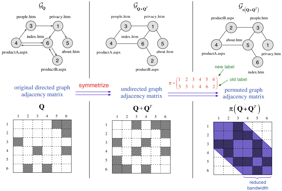
Figure 4 A simplified version of SimRank minimum bandwidth ordering problem with permutation \pi on the adjacency matrix \mathbf{Q} .
