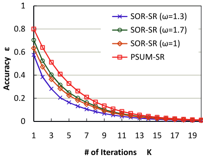
(c) Convergence Rate ( n = 10K )
