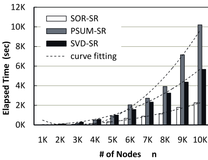
(a) Time Efficiency on Sparse Graphs
