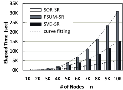
(b) Time Efficiency on Dense Graphs
