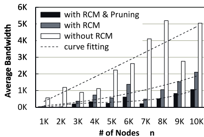
(e) I/O Efficiency on Sparse Graphs
