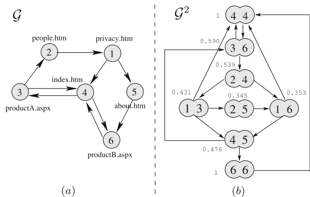
Figure 1 SimRank propagating similarity from pair to pair in \mathcal{G} associated with the propagation from node to node in \mathcal{G}^2 with a decay factor c = 0.8 .
