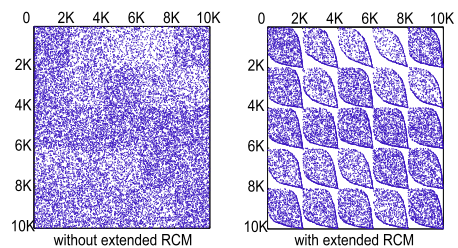
(f) Extended RCM ( m = 5,496,208 )
