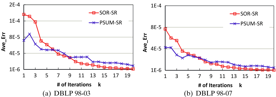
Figure 8 Effectiveness on DBLP datasets.
