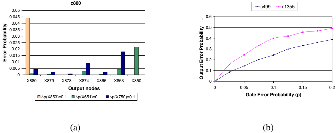
Fig. 7. (a) Sensitivity of output error probability with respect to individual gate errors for c880 (b) Output error profiles of two alternative logic implementation (c499 and c1355)
