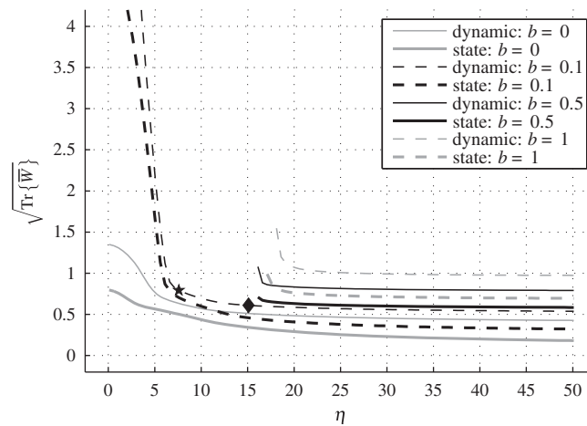
Figure 2. Trade-off between the imposed upper bound \eta on \|T_{uw}\|_\infty and the guaranteed upper bound \sqrt{\text{Tr}\{\bar{W}\}} on \|T_{yw}\|_2 . Comparison between gain-scheduled state feedback (thick) and dynamic output feedback (thin).
