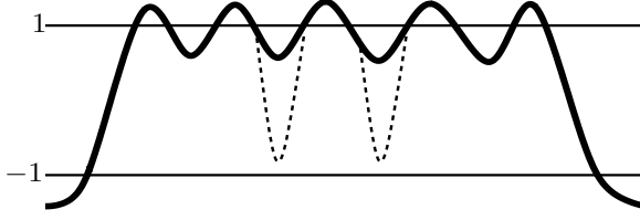
Figure 1: Sketch of four different periodic solution u \in [\sigma_1^2 \sigma_2^{10}, 10] . The solid black curve represents one solution. The second (third) solution is obtained by replacing the second (third) dip with the dashed curve. The fourth solution is the one for which both dips are replaced by the dashed curves.
