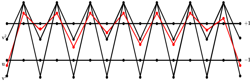
Figure 7: The braid class [\mathbf{u} \text{ rel } \mathbf{w}] \in \mathcal{D}_{14}^1 \text{ rel } \mathbf{w} for I = \{2, 4, 5\} . The skeletal strand v^3 is not displayed.
