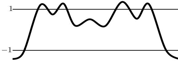
Figure 9: Sketch of a periodic solution u \in [\sigma_1^2 \sigma_2^8, 10] .
