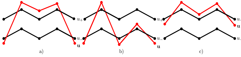
Figure 15: Representants of the three different relative braid classes. A fixed point in the relative braid class defined by its representant a) corresponds to the solution of the type I, b) type II and c) type III. Braid classes (a) and (b) are proper but (c) is not.
