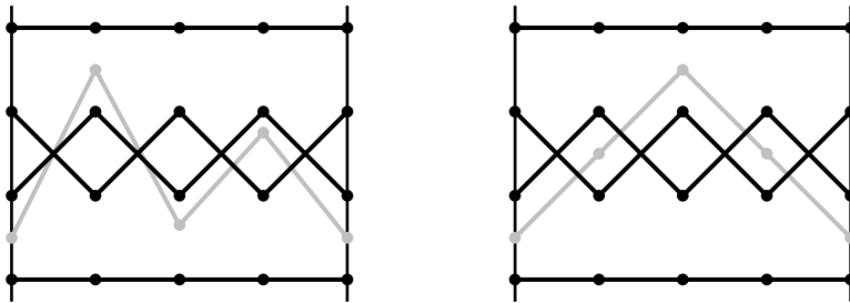
Figure 13: Non-proper [left] and proper [right] relative braid classes. Both classes are bounded.
