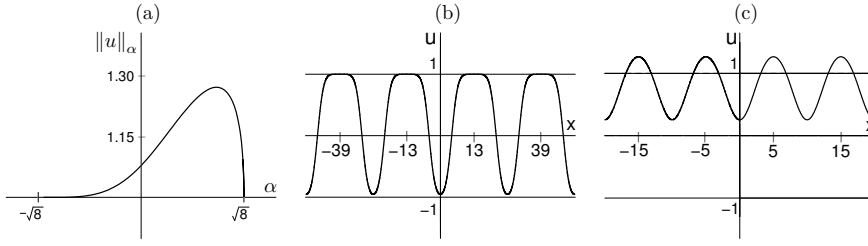
Figure 2: Bifurcation diagram for the solutions of the third type and corresponding solutions which are in the class \mathbf{u}_{1,1} . Solution (b) corresponds to \alpha = -1 and (c) to \alpha = 1 .
