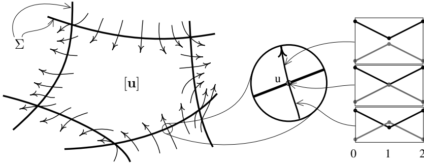
Figure 11: A schematic picture of a parabolic flow on a braid class. The boundary of the braid class is contained in the set of singular braids \Sigma .
