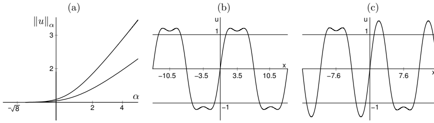
Figure 2: Bifurcation diagram for the solutions of the first type and corresponding solutions for \alpha = 1.5 . The number of monotone laps for the solution pictured at (b) is six and it intersects u_\pm two times. For solution (c) number of monotone laps is ten and crossing number with u_\pm is six.
