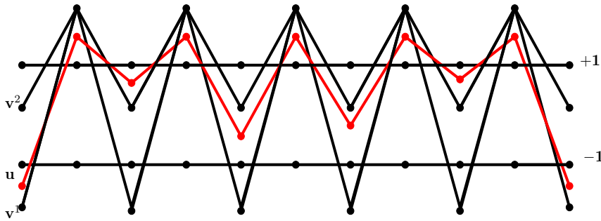
Figure 6: The braid class [\mathbf{u} \text{ rel } \mathbf{w}] \subset \mathcal{D}_{10}^1 \text{ rel } \mathbf{w} for I = \{2, 3\} with the simplified skeleton. To keep the figure clear we do not display the strand \mathbf{v}^3 which makes the braid class bounded.
