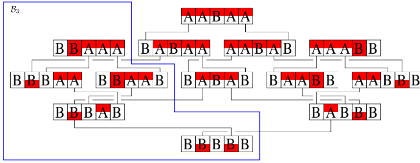
Figure 9: Schematic representation of U(3) . The shaded faces form U^-(3) . The cubes in the polygon form \mathcal{B}_3 and the other cubes form \mathcal{A}_3 .
