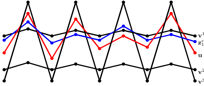
Figure 7: A representat of the braid class [\mathbf{u} \text{ rel } \mathbf{v}^\varepsilon] for p = 4, q = 3, p' = 1 and q' = 2 . If we skip the strand z_1^\varepsilon from the skeleton we get a representant of the braid class [\mathbf{u} \text{ rel } \mathbf{v}] .
