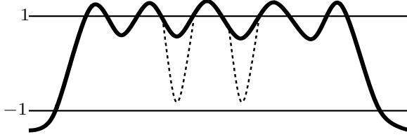
Figure 8: Sketch of four different periodic solution u \in [\sigma_1^2 \sigma_2^{10}, 10] . The solid black curve represents one solution. The second (third) solution is obtained by replacing the second (third) dip with the dashed curve. The fourth solution is the one for which both dips are replaced by the dashed curves.
