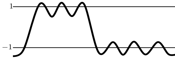
Figure 20: Sketch of a periodic solutions of the class [\sigma_1^8 \sigma_2^6, 12] .
