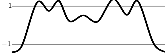
Figure 2: Sketch of a periodic solution u \in [\sigma_1^2 \sigma_2^8, 10] .
