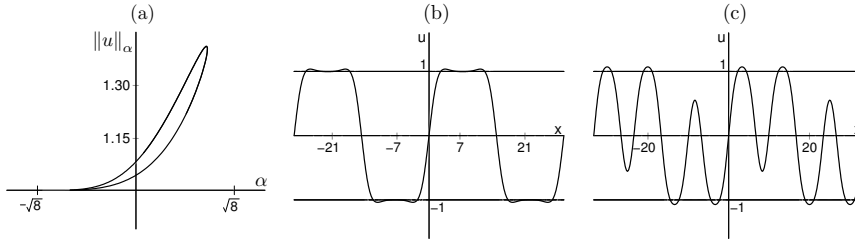
Figure 6: Bifurcation diagram for the solutions of the second type and corresponding solutions. Both solutions in (b) and (c) lie on the same bifurcation branch and have six monotone laps and crosses u_{\pm} four times. These solutions corresponds to the parameter value \alpha = -\frac{1}{10} .
