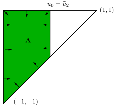
Figure 6: The triangle D = [-1, 1] \times [-1, 1] \setminus \{u_1 > u_0\} . The arrows denote (schematically) the direction of the gradient \nabla W_2 . Clearly W_2 has a maximum on A .
