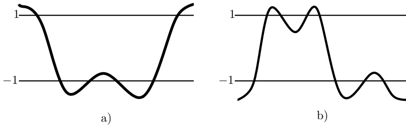
Figure 18: Sketch of periodic solutions; a) of the class [\sigma_2^2 \sigma_1^4, 4] ; b) of the class [\sigma_1^4 \sigma_2^4, 4] .
