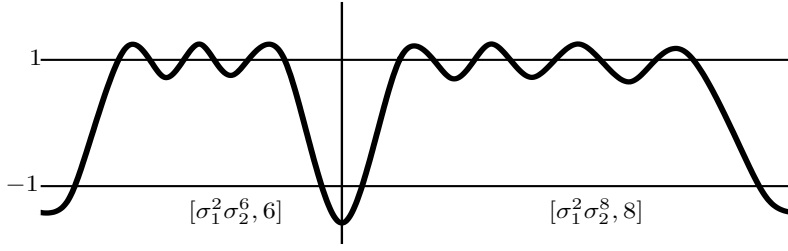
Figure 7: Sketch of aperiodic solution u \in [\sigma_1^2 \sigma_2^6 \sigma_1^2 \sigma_2^8, 14] which consists of two blocks namely [\sigma_1^2 \sigma_2^6, 6] and [\sigma_1^2 \sigma_2^8, 8] .
