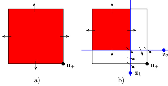
Figure 5: Figure (a) schematically shows behavior of the vector field \mathcal{R} on the boundary of the non-proper braid class [\mathbf{u} \text{ rel } \mathbf{v}]_{\mathcal{E}} corresponding to the third type of solution. The strand \mathbf{u}_+ is a fixed point for the flow \Psi^t and some trajectories approach this point as t \rightarrow -\infty . Figure (b) shows the behavior of the perturbed vector field on the boundary of the proper braid class [\mathbf{u} \text{ rel } \bar{\mathbf{v}}]_{\mathcal{E}} , where \bar{\mathbf{v}} = \mathbf{v} \cup \mathbf{z}_1 \cup \mathbf{z}_2 and \mathbf{z}_1, \mathbf{z}_2 are fixed strands for this perturbed vector field.
