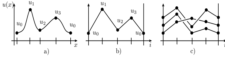
Figure 10: (a) A periodic function and (b) its piecewise linear graph (c) a braid consisting of 3 strands.
