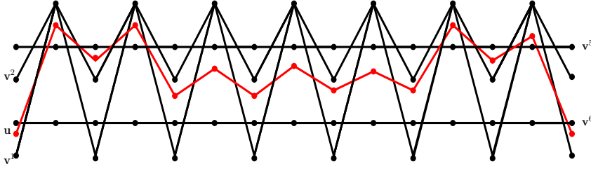
Figure 12: A representative of the braid class [\mathbf{u} \text{ rel } \mathbf{w}]_I \in \mathcal{E}_{14}^1 \text{ rel } \mathbf{w} for q = 3 and I = \emptyset
