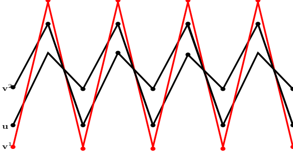
Figure 3: Sketch of the strands v^1, v^2 and v^3 .
