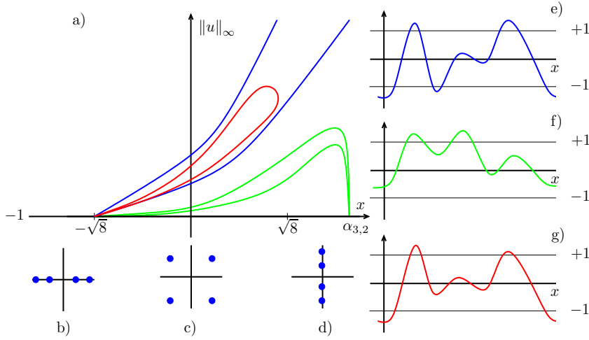
Figure 1: Bifurcation diagram a) shows three different types of the branches, in the plane (\alpha, \|u\|_\infty) , which bifurcate for \alpha = -\sqrt{8} . Solutions on the branches that extend beyond the boundary of the diagram are of the first type, see e) for an example; branches that form closed loops consist of solutions of the second type, see f) for an example; branches collapsing on \|u\|_\infty = 1 consist of solutions of the third type see, g) for example. The spectrum of the linearization around P_+ and P_- for b) \alpha \leq -\sqrt{8} ; c) \alpha \in (-\sqrt{8}, \sqrt{8}) ; d) \sqrt{8} \leq \alpha .
