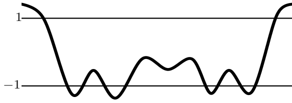
Figure 19: Sketch of a periodic solutions of the class [\sigma_2^2 \sigma_1^8, 10] .
