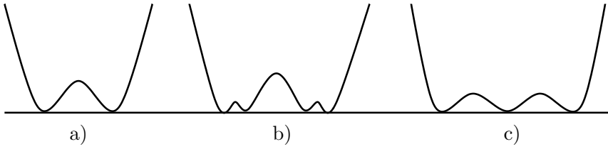
Figure 17: Figure a) Potential F(u) = \frac{1}{4}(u^2 - 1)^2 ; b) small perturbation of F(u) ; c) potential with three wells.
