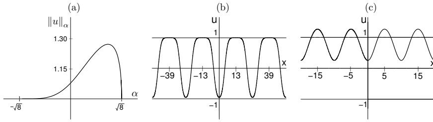
Figure 3: Bifurcation diagram for the solutions of the third type and corresponding solutions which are in the class [\sigma_2^2, 2] . Solution (b) corresponds to \alpha = -1 and (c) to \alpha = 1 .
