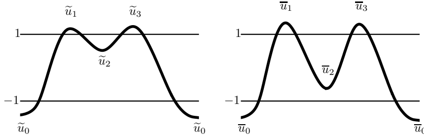
Figure 4: Sketch of two periodic solutions \tilde{u}, \bar{u} \in [\sigma_1^2 \sigma_2^4, 4] . Their extremal points are labeled by \tilde{u}_i and \bar{u}_i .
