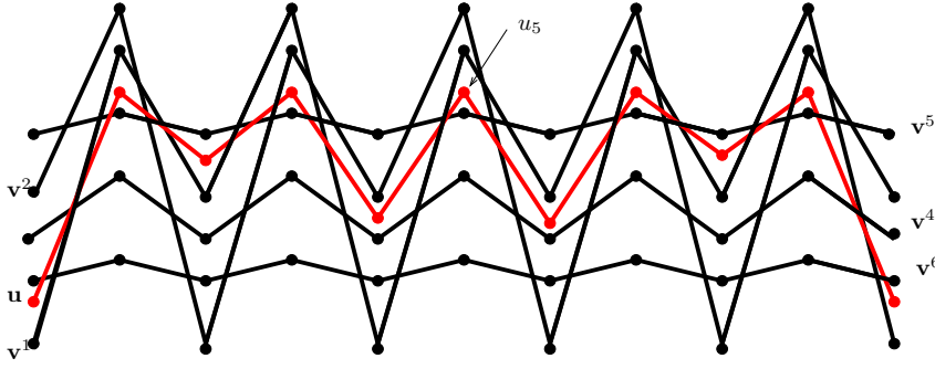
Figure 4: A representative of the braid class [\mathbf{u} \text{ rel } \mathbf{w}]_{\mathcal{E}} \subset \mathcal{E}_{10}^1 \text{ rel } \mathbf{w} for I = \{2, 3\} . To keep the figure synoptical we do not display the skeletal strand \mathbf{v}^3 . The strand \mathbf{v}^3 makes the braid class [\mathbf{u} \text{ rel } \mathbf{w}]_{\mathcal{E}} bounded. There would be no upper bound for u_5 without the strand \mathbf{v}^3 .
