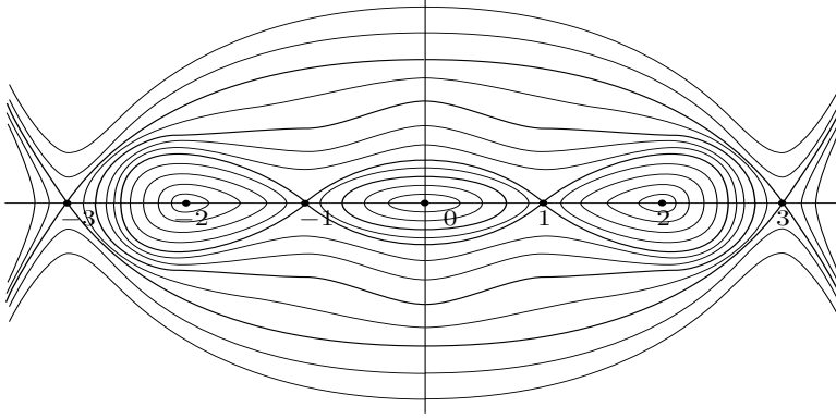
Figure 8: The integrable model in the (u, u_t) plane; there are centers at 0, \pm 2 and saddles in \pm 1, \pm 3 .
