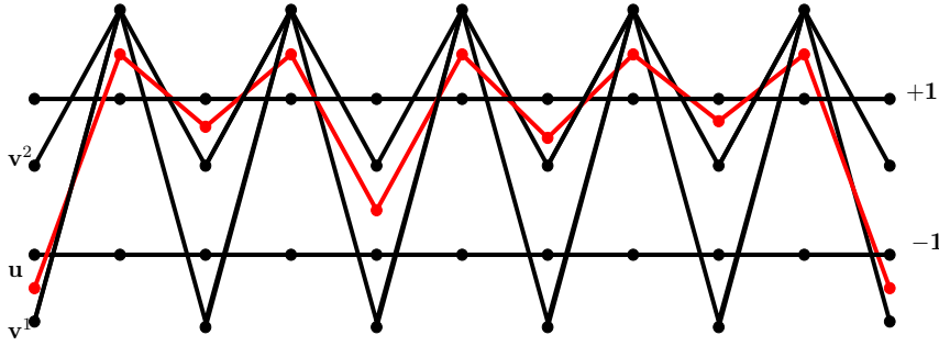
Figure 5: The braid class [\mathbf{u} \text{ rel } \mathbf{w}] \subset \mathcal{D}_{10}^1 \text{ rel } \mathbf{w} for I = \{2\} . The skeletal strand \mathbf{v}^3 is not displayed.
