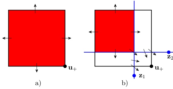
Figure 16: Figure (a) schematically shows behavior of the vector field \mathcal{R} on the boundary of the non-proper braid class [\mathbf{u} \text{ rel } \mathbf{v}]_{\mathcal{E}} corresponding to the third type of solution. The strand \mathbf{u}_+ is a fixed point for the flow \Psi^t and some trajectories approach this point as t \rightarrow -\infty . Figure (b) shows the behavior of the perturbed vector field on the boundary of the proper braid class [\mathbf{u} \text{ rel } \bar{\mathbf{v}}]_{\mathcal{E}} , where \bar{\mathbf{v}} = \mathbf{v} \cup \mathbf{z}_1 \cup \mathbf{z}_2 and \mathbf{z}_1, \mathbf{z}_2 are fixed strands for this perturbed vector field.
