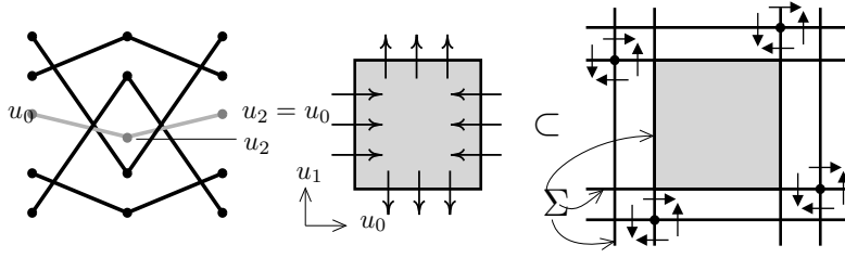
Figure 14: A representant of the relative braid class [\mathbf{u} \text{ rel } \mathbf{v}] \subset \mathcal{D}_2^1 \text{ rel } \mathbf{v} with four skeleton strands (black) and one free strand (gray). Sketch of the flow \Psi^t at the boundary is shown in the middle. At the right we present a bigger portion of the space \mathcal{D}_2^1 \text{ rel } \mathbf{v} to show the direction of the flow in the neighborhood of fixed points corresponding to the skeleton \mathbf{v} . The braid classes adjacent to these fixed points are not proper.
