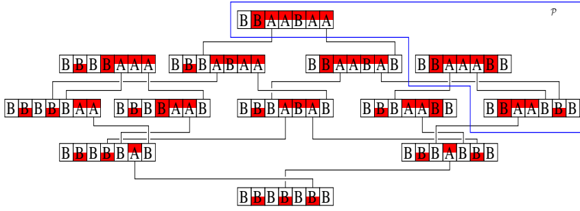
Figure 10: Schematic representation of \mathcal{B}_4 . The shaded faces form \mathcal{B}_4^- . The cubes in the polygon form \mathcal{P} and the cubes out of it form \mathcal{Q} .
