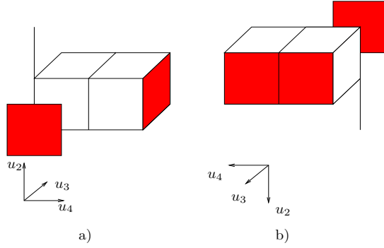
Figure 11: a) b) the projection of the set \mathcal{A}_3^- \cap \mathcal{B}_3^- on the coordinates (u_2, u_3, u_4) . The set \mathcal{P}_1^- \cap \mathcal{Q}_1^- is shaded.
