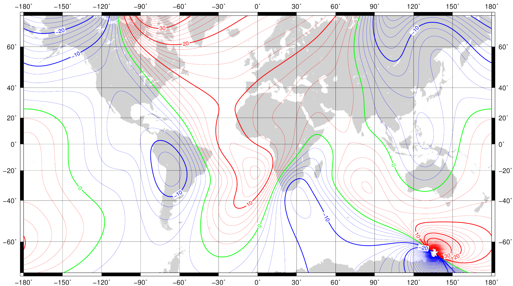
Annual rate of change of declination for 2020.0 to 2025.0 from the World Magnetic Model (WMM2020). Red – easterly change, blue – westerly change, green – zero change. Contour interval is 2'/year, white star is location of a magnetic pole and projection is Mercator. This is an example of an isoporic chart. Credit: British Geological Survey (UK Research and Innovation).
