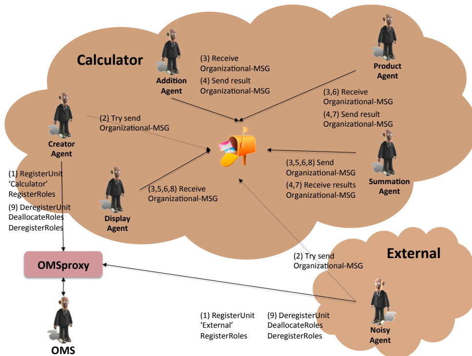
Figure 8.12: Organizational Message Example diagram
