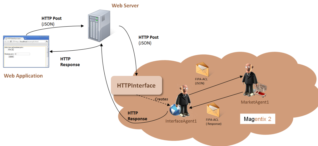
Figure 9.1: HTTP Interface framewok
