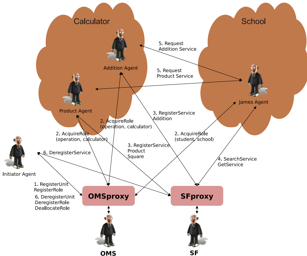
Figure 8.9: Thomas Example diagram
