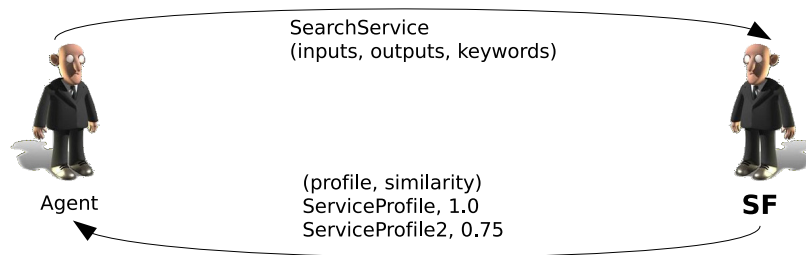
Figure 8.7: Agent interaction protocol to search service.
