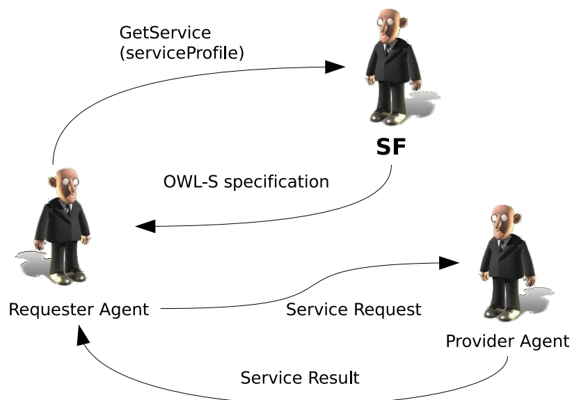
Figure 8.8: Agent interaction protocol to request a service.
