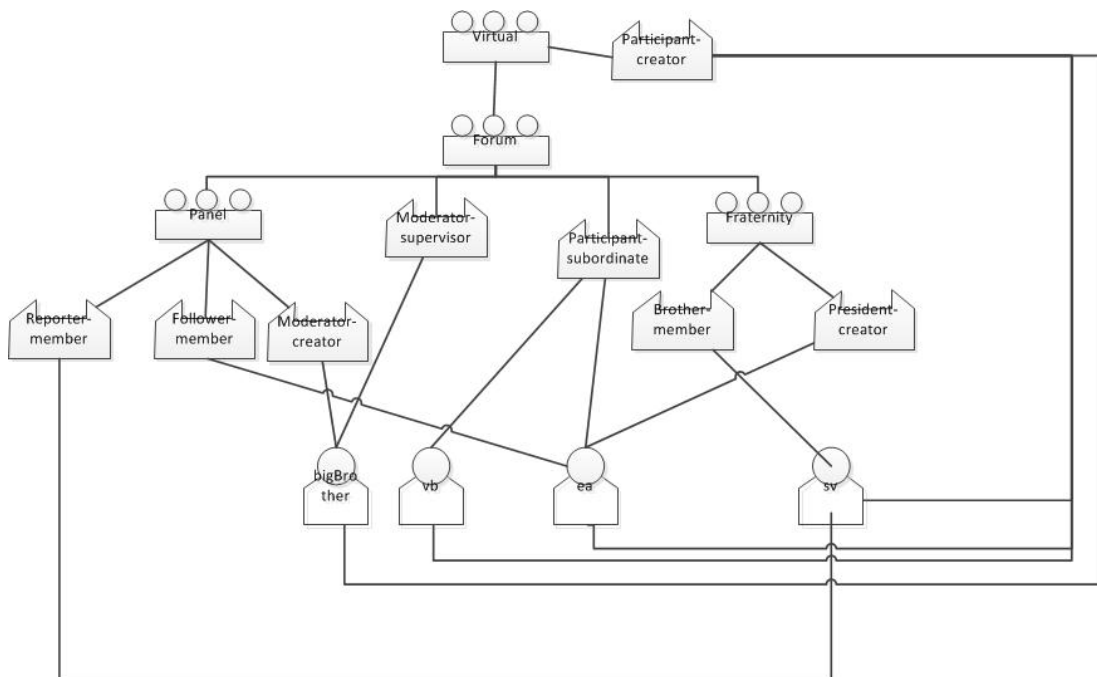
Figure 8.2: Organizational view of the form example: organizations, roles and agents
