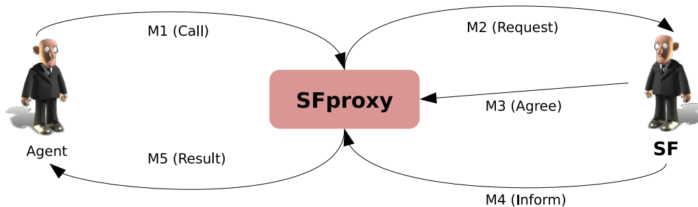
Figure 8.4: Interaction between user agent and SF agent through the SFProxy
