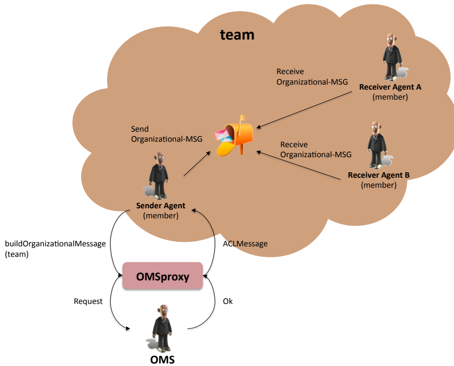
Figure 8.10: Organizational messaging: Example diagram.
