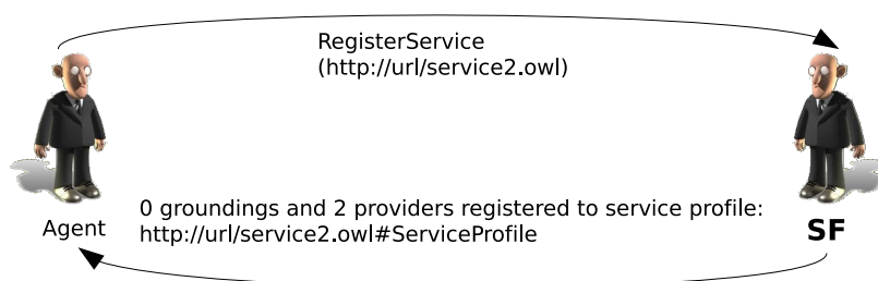
Figure 8.6: Agent interaction protocol to register new providers.
