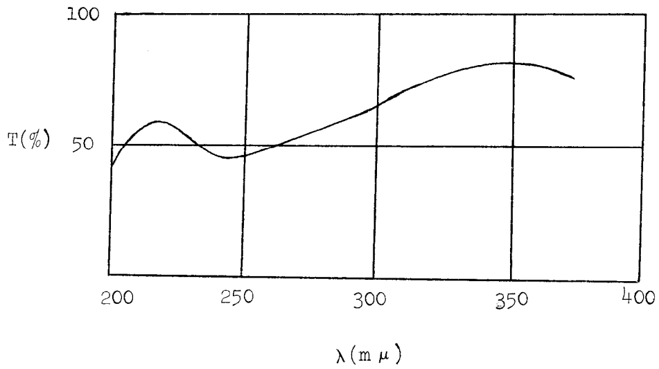
Figure 3.3-2 - UV Lens Spectral Transmission
