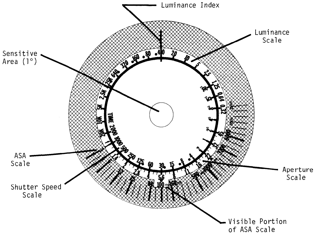
Figure 6.1-3 - Spotmeter Scales
