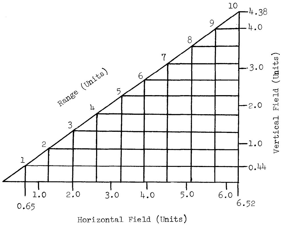
Figure 3.2-1 - 55 mm. Visible Lens and Field-of-view Chart
