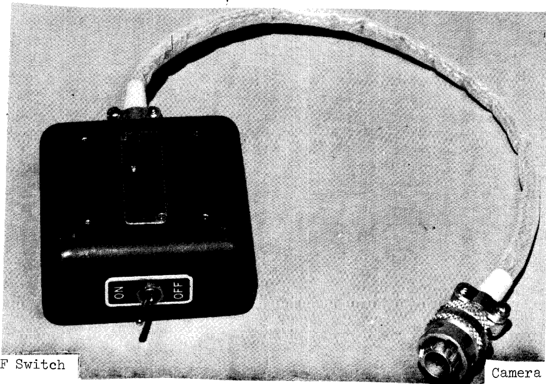
Figure 4.14-1 - 20-Second Intervalometer (-301)
