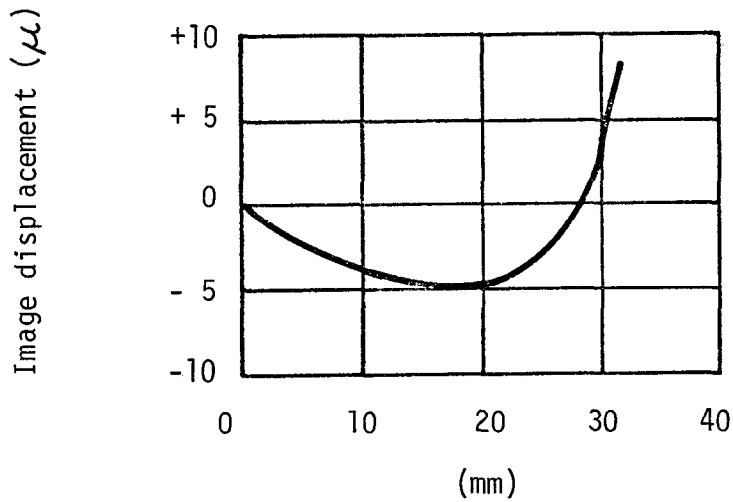
Figure 4.3-3 - 60 mm. Lens Radial Distortion (Typical)
