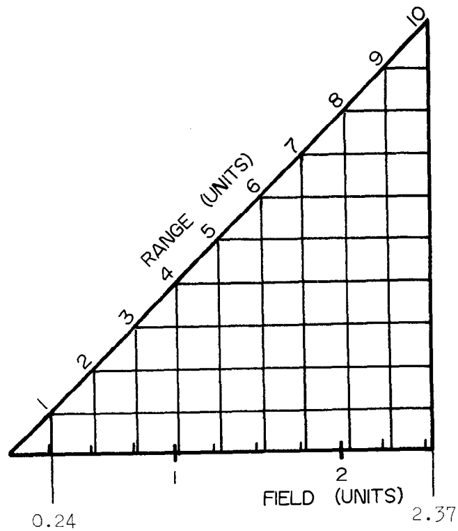
Figure 4.11-1 - 250 mm. Lens and Field-of-View Chart
