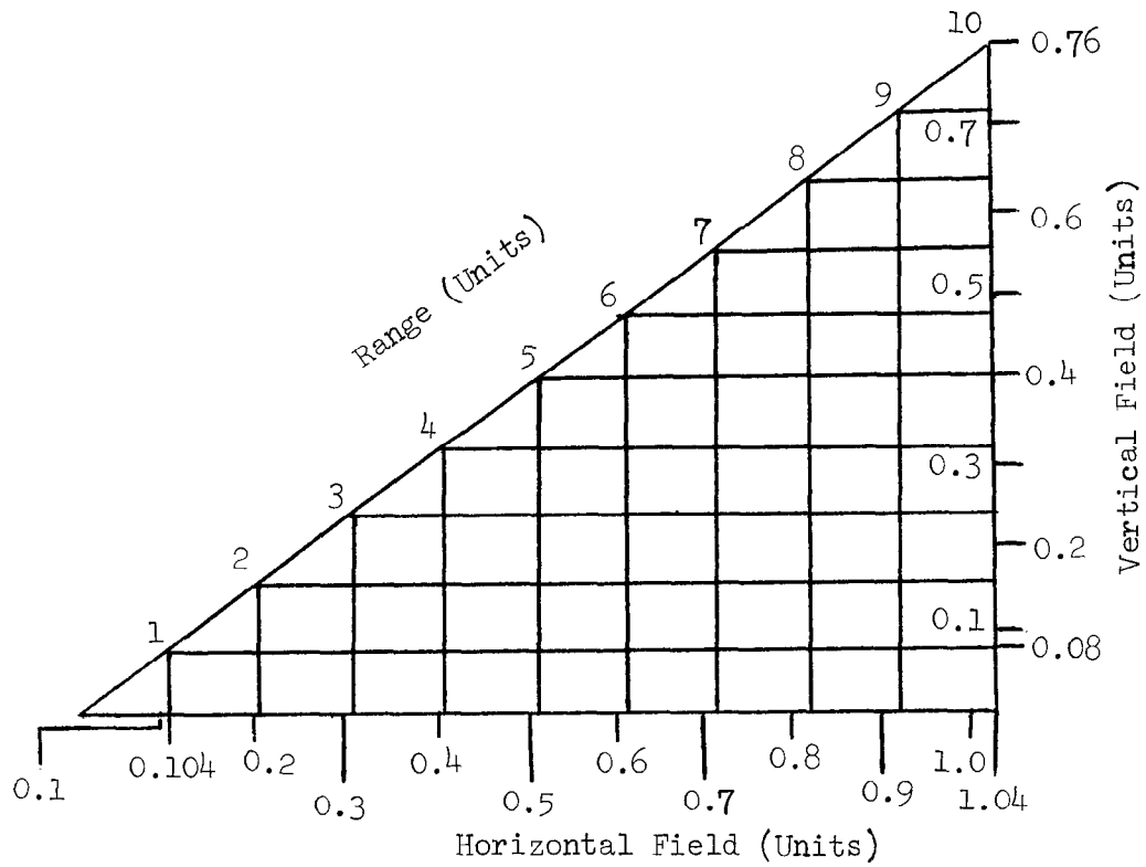
Figure 2.10-1 - 100 mm. Lens (-202) and Field-of-view Chart
