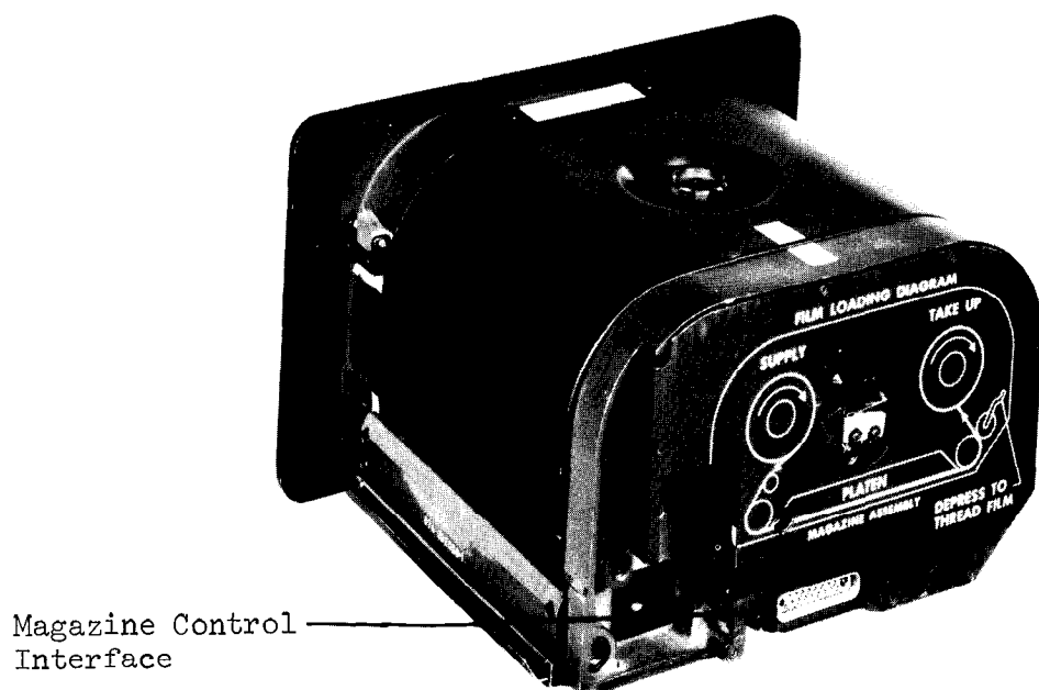
Figure 5.2-2 - ETC Magazine, Rear View
