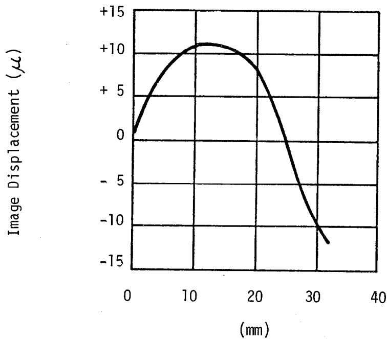
Figure 4.5-2 - 100 mm. Lens Radial Distortion (Typical)
