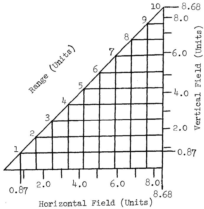
Figure 4.3-1 - 60 mm. Lens and Field-of-view Chart
