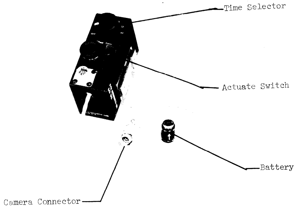
Figure 3.6-1 - NK Timer
