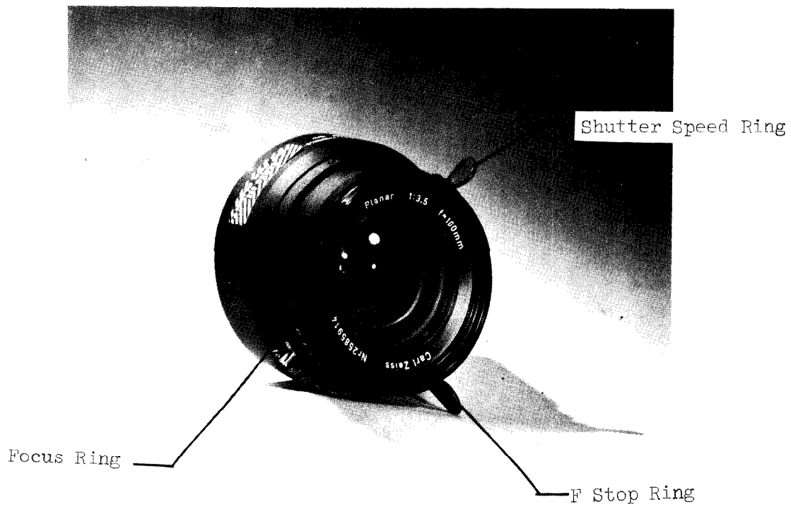
Figure 4.5-1 - 100 mm. Lens
