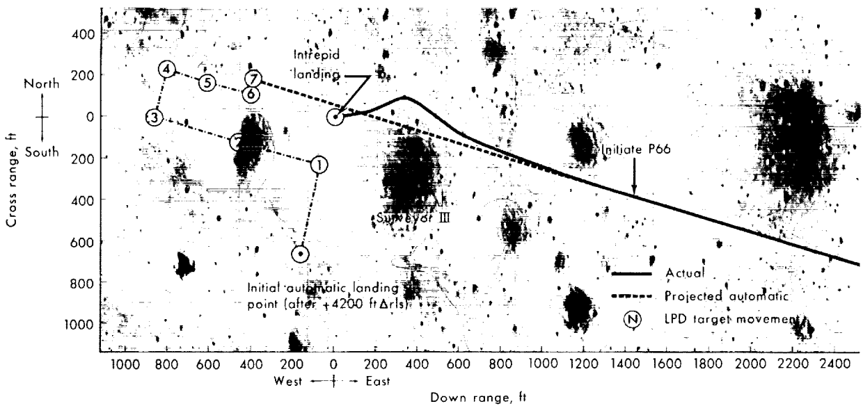
Figure 33. - Apollo 12 approach phase.
