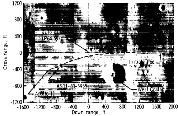
Figure 23. - Apollo 11 groundtrack for the landing phase.
