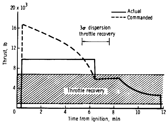
(a) Thrust.
