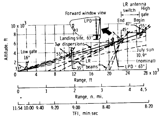
Figure 9. - Approach phase.
