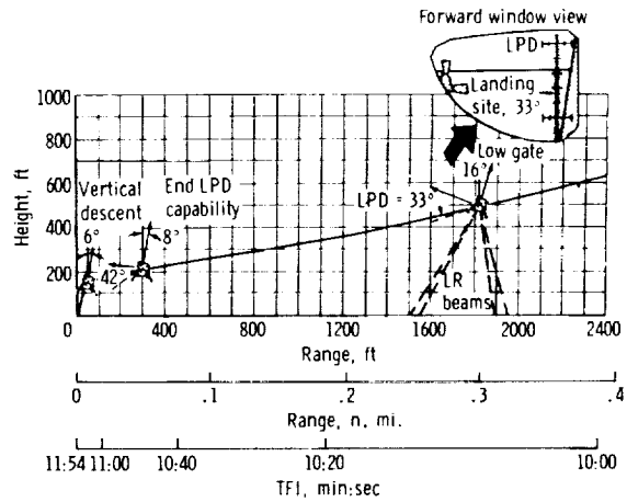
Figure 10. - Landing phase.
