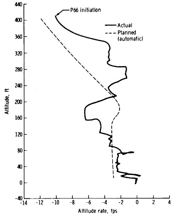
Figure 25. - Apollo 11 altitude as a function of altitude rate for the landing phase.
