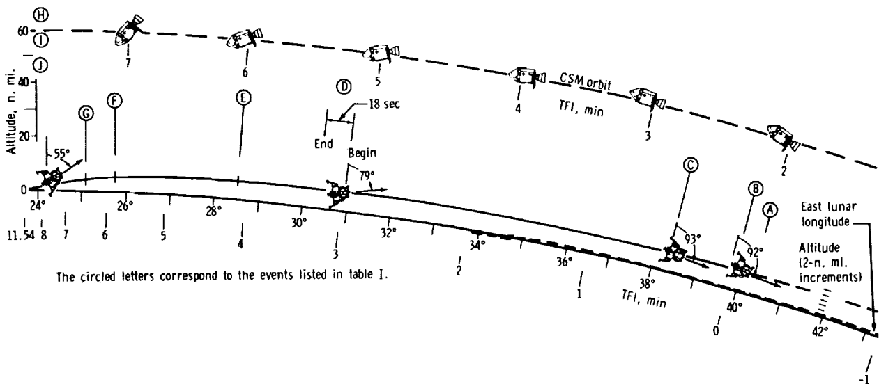
Figure 7. - Premission Apollo 11 LM powered descent.
