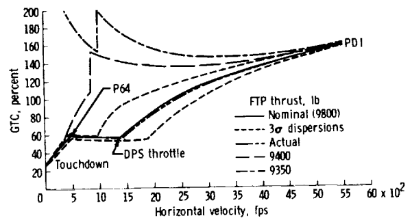
Figure 17. - Guidance thrust command as a function of horizontal velocity.
