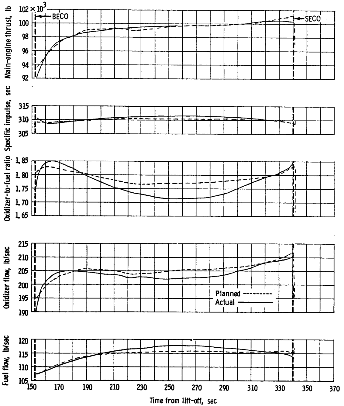
Figure 5.2-2 - Stage II engine performance.
