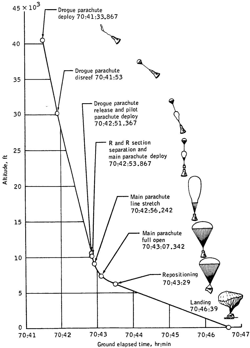
Figure 5.1.11-1. - Landing system performance.
