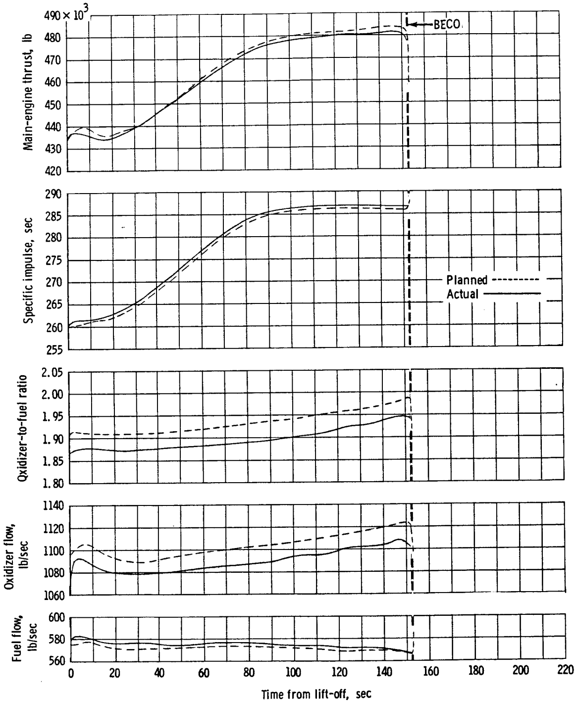
Figure 5.2-1. - Stage I engine performance.
