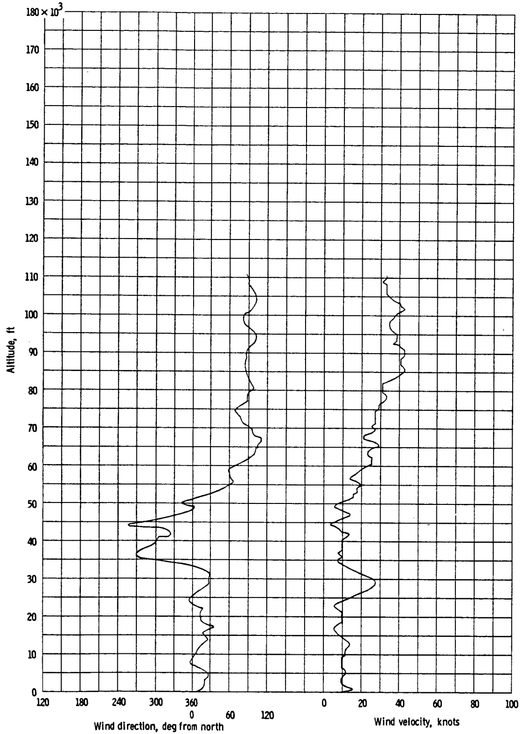
Figure 12.2-1. - Variation of wind direction and velocity with altitude for the GAATV at 20:39 G.m.t., July 18, 1966.
