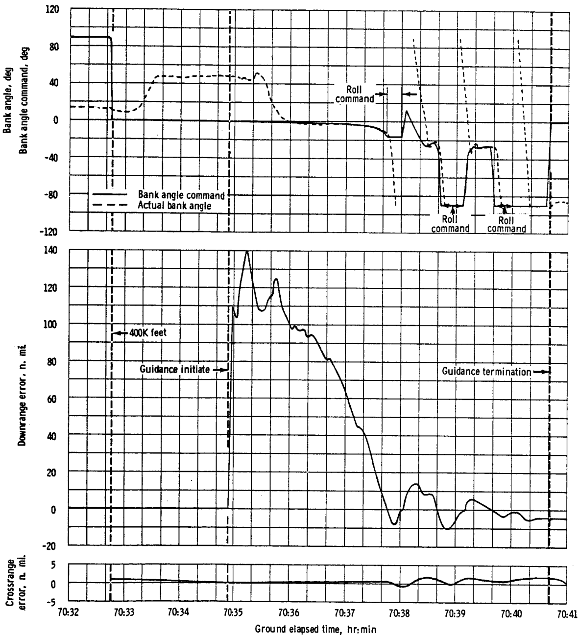
Figure 5.1.5-24. - Reentry guidance parameters.
