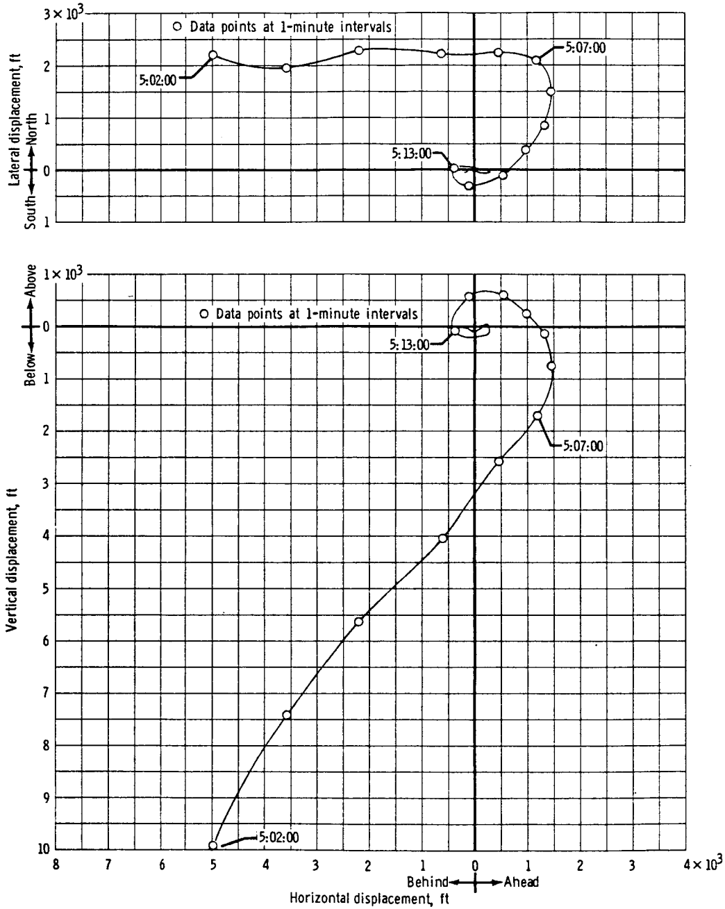
Figure 5.1.5-15. - First rendezvous final approach.
