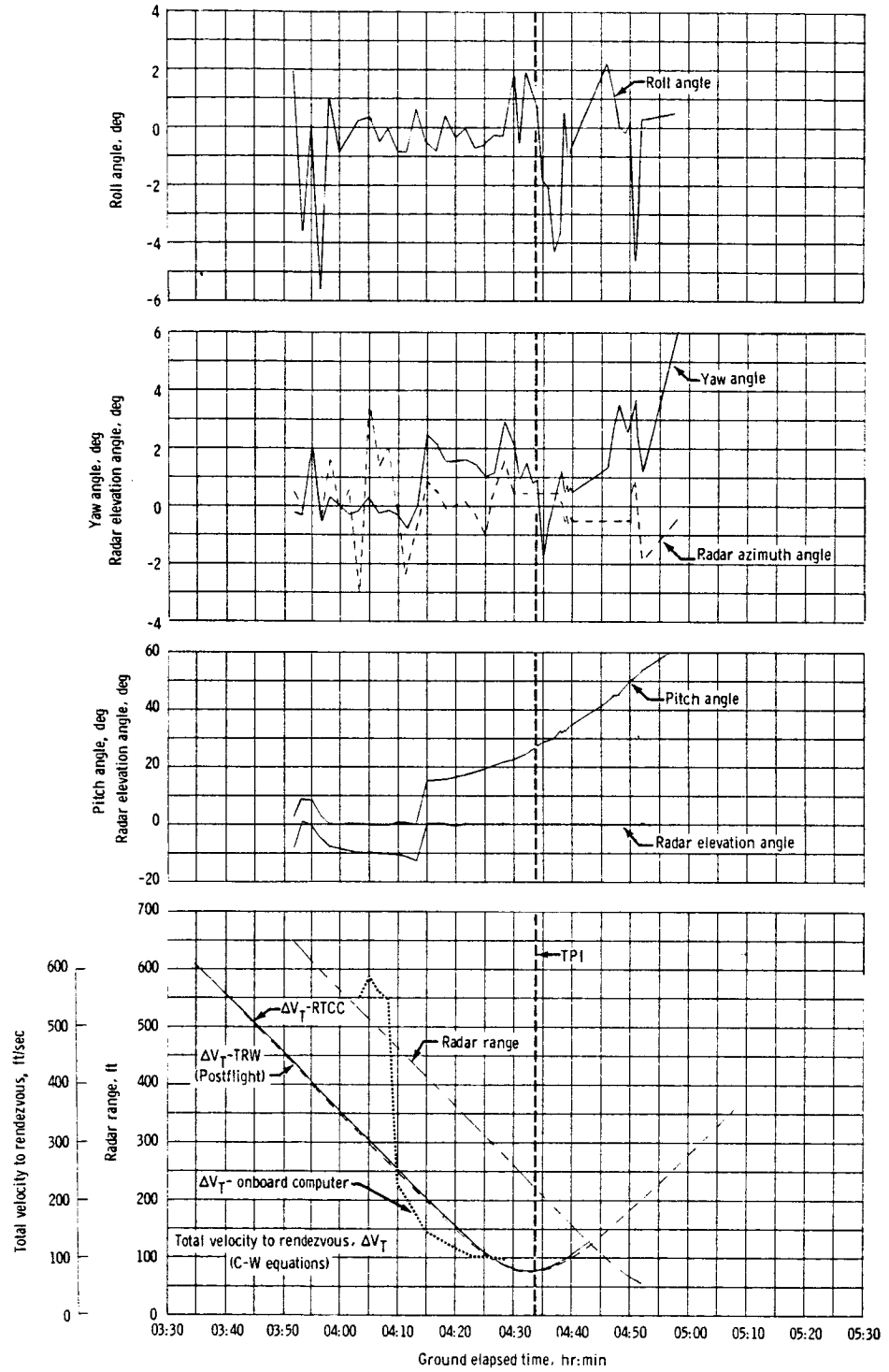
Figure 5.1.5-8. - Computer data for the closed-loop rendezvous.
