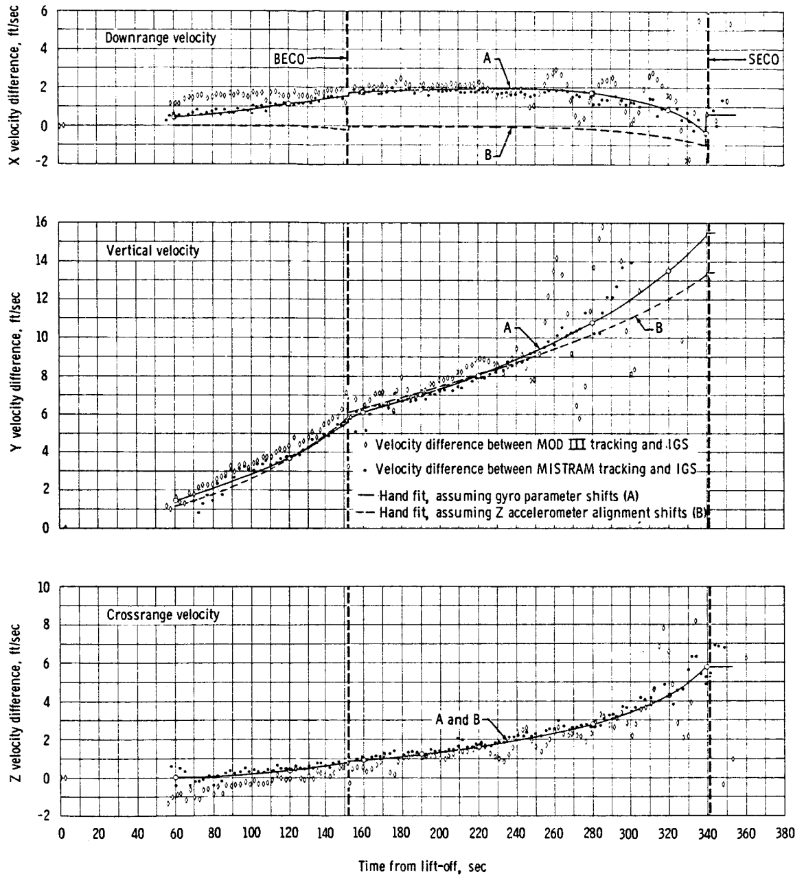
Figure 5.1.5-3. - Comparisons of spacecraft IGS and radar tracking velocities.
