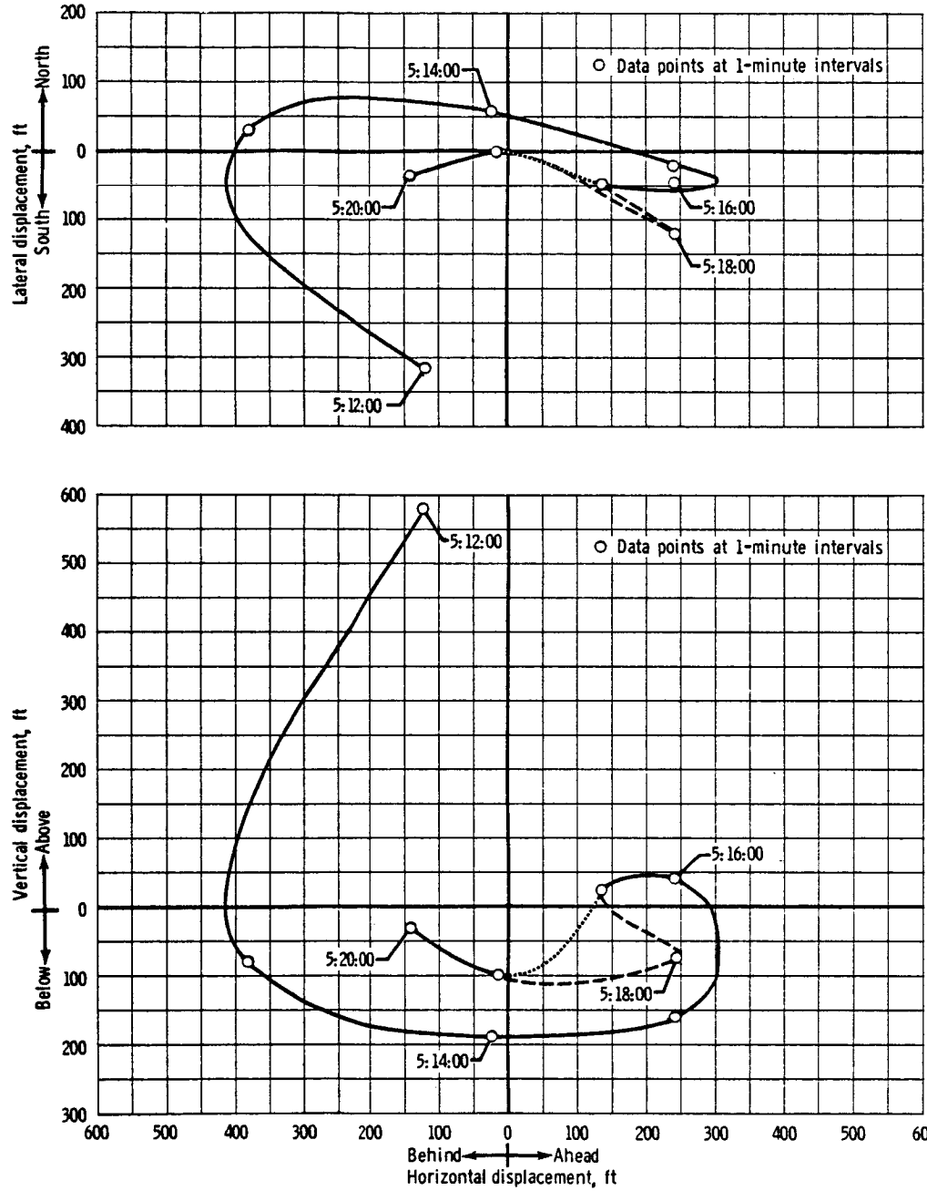
Figure 5.1.5-16. - First rendezvous final approach (expanded scale).
