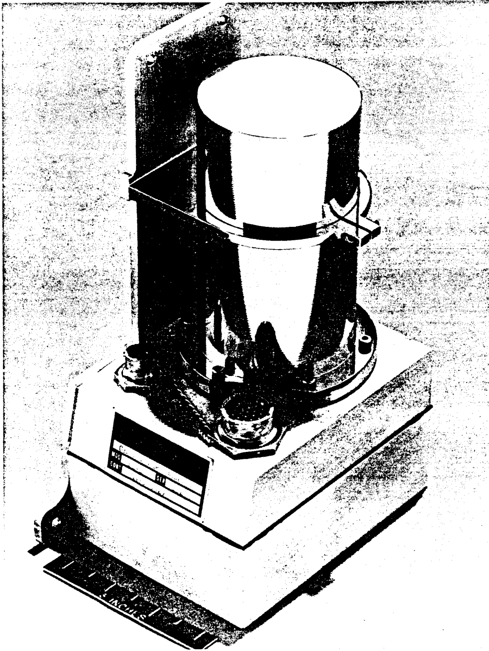
Figure 8.5-1. - Experiment M409, bremsstrahlung spectrometer.
