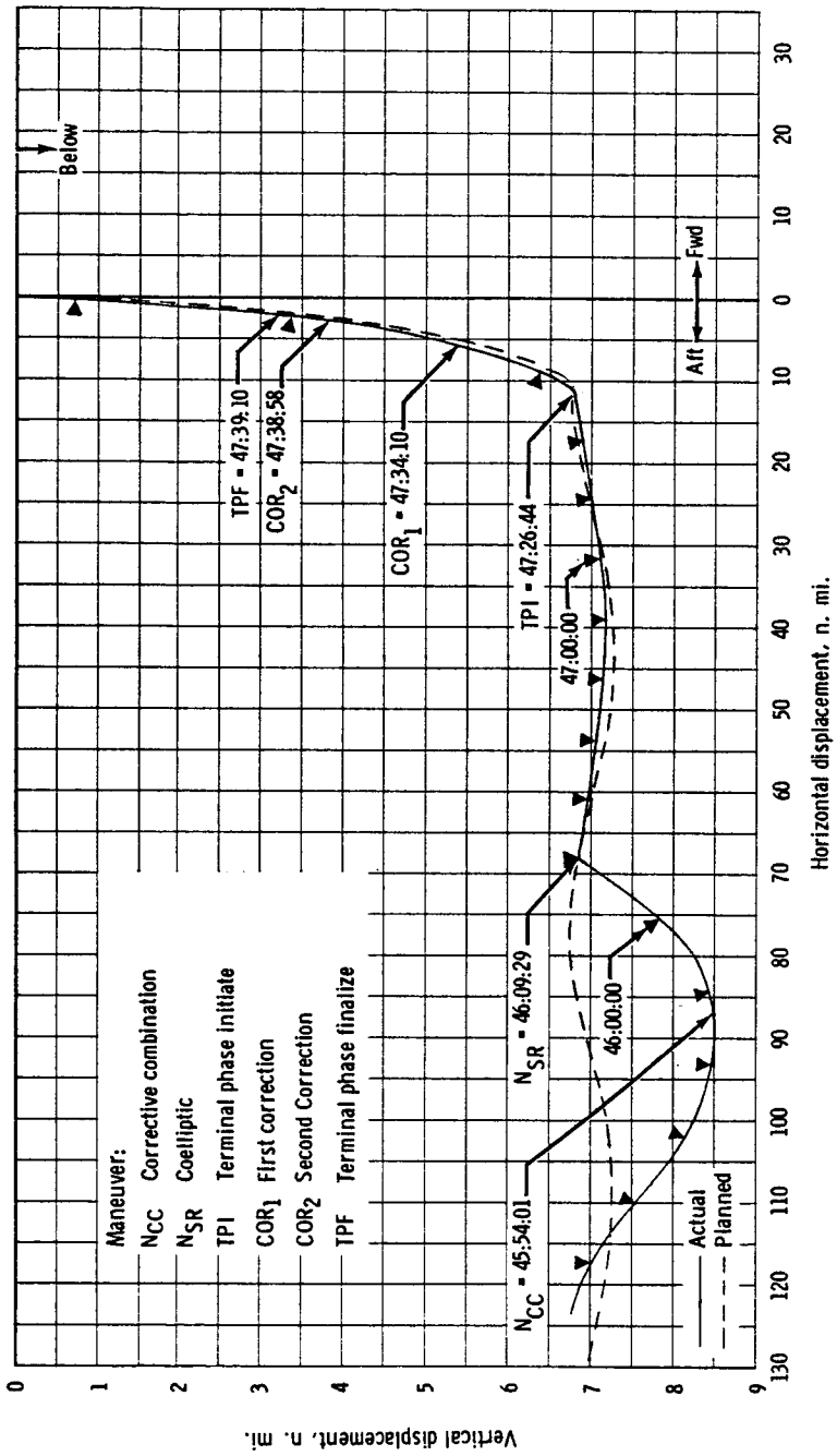
(c) Relative trajectory profile of second rendezvous from Gemini VIII GATV to Spacecraft 10 in curvilinear coordinate system.
