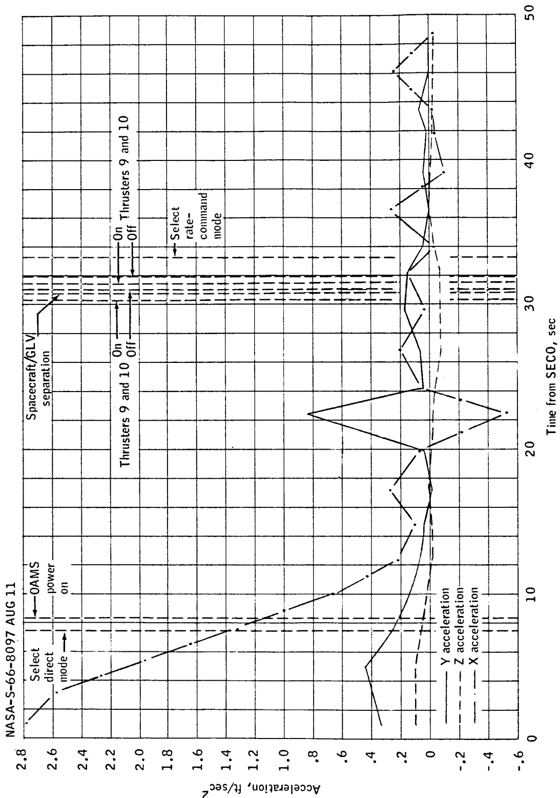
Figure 5.1.5-2. - Spacecraft acceleration measured after SECO.
