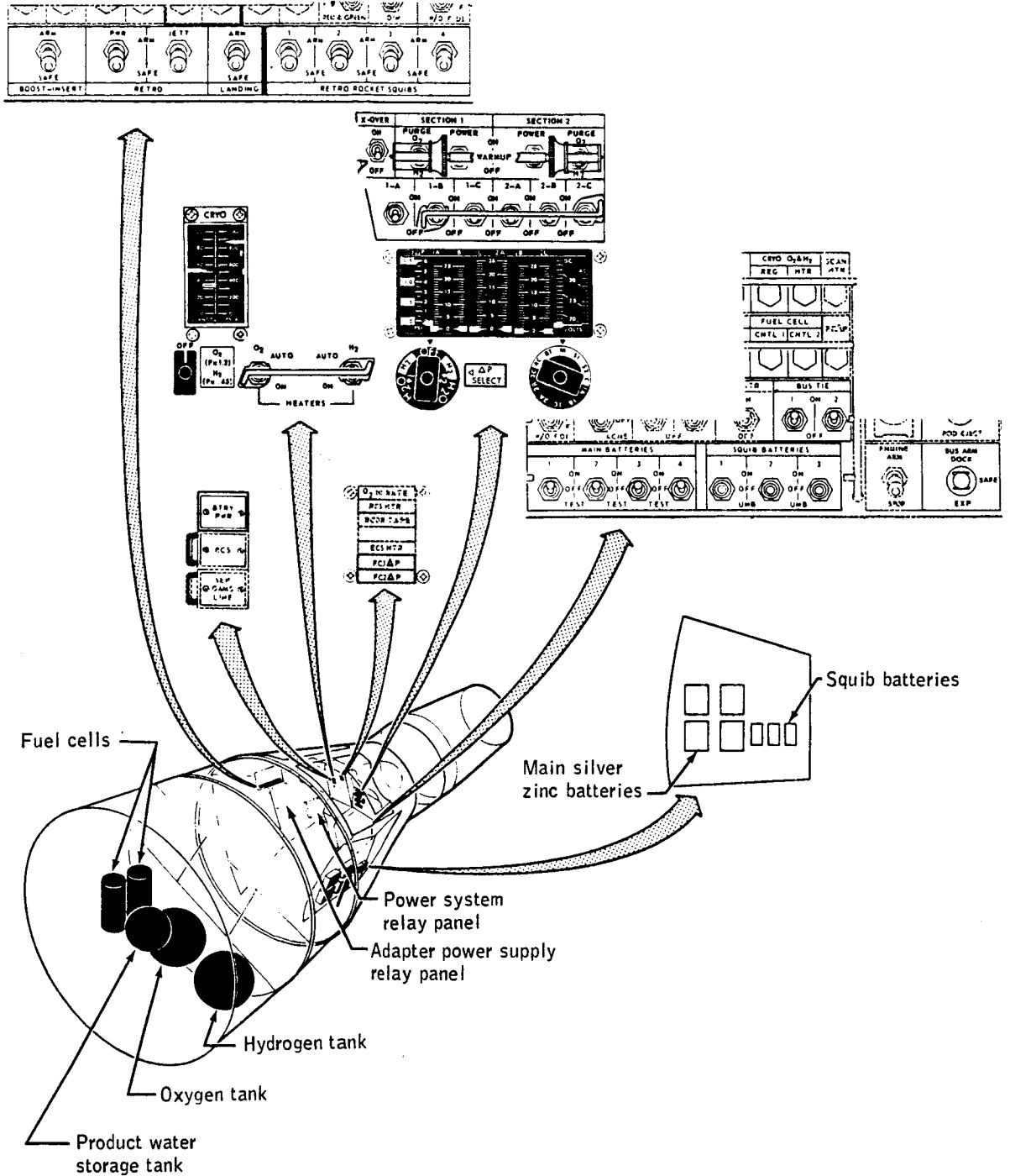
Figure 3.1-2. - Electrical system.
