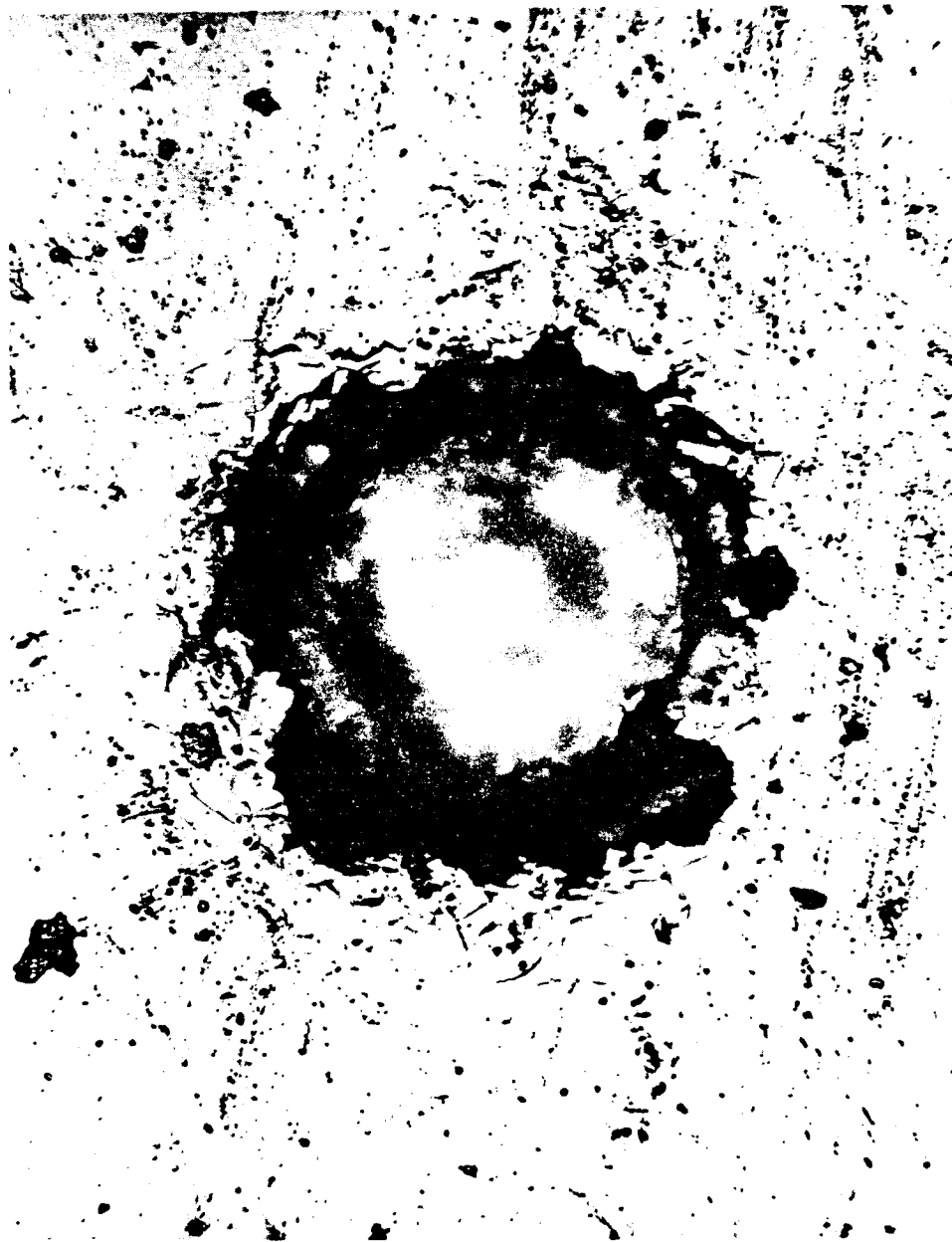
Figure 8.11-3. - Experiment S010 micrometeorite crater, 400 - micron diameter.
