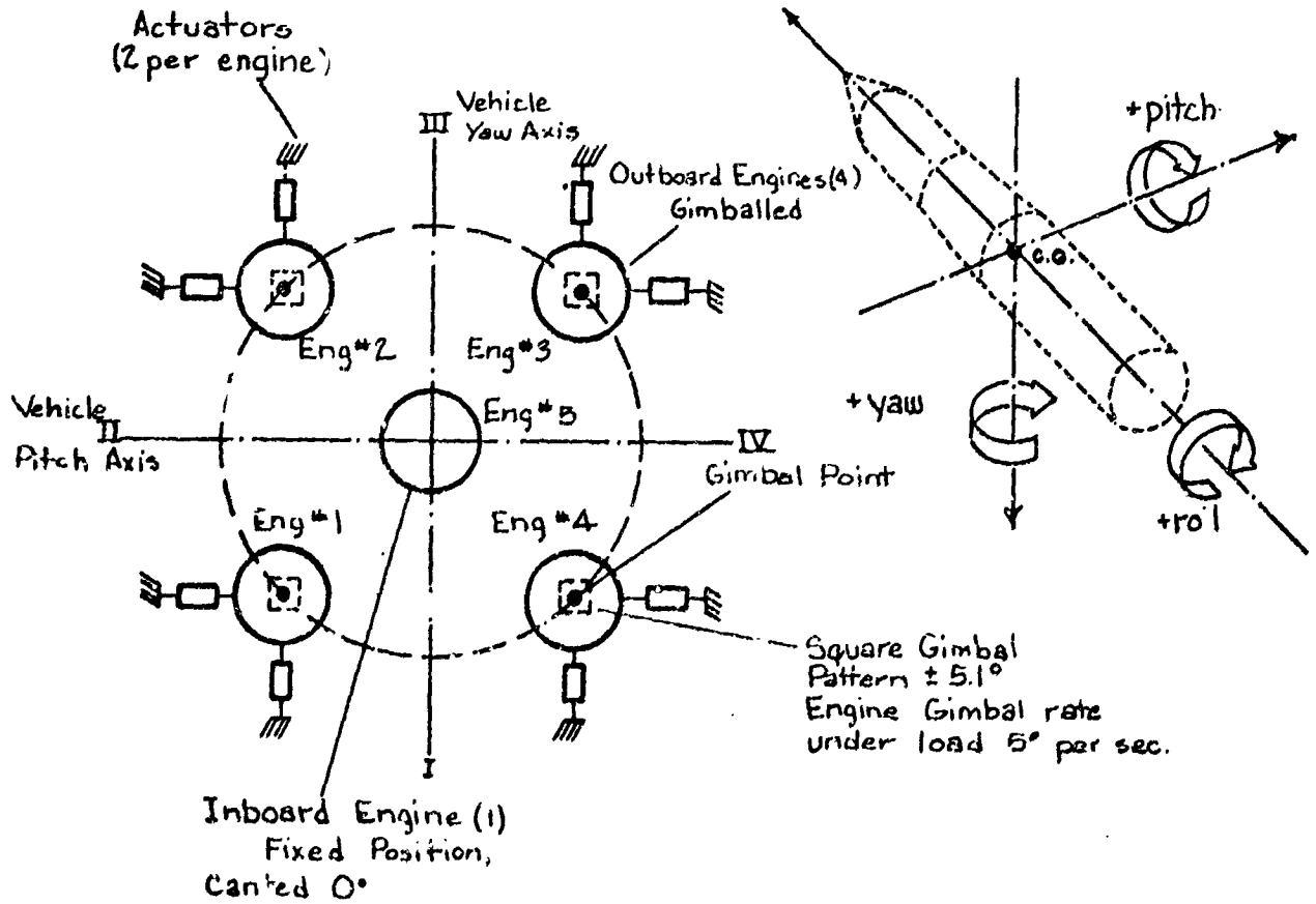
S-IC Thrust Vector Control System
