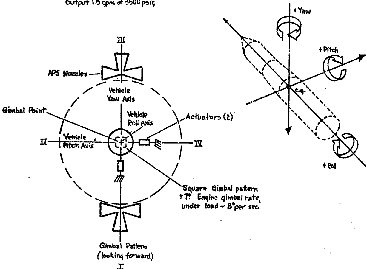
S-108 Thrust Vector Control System
