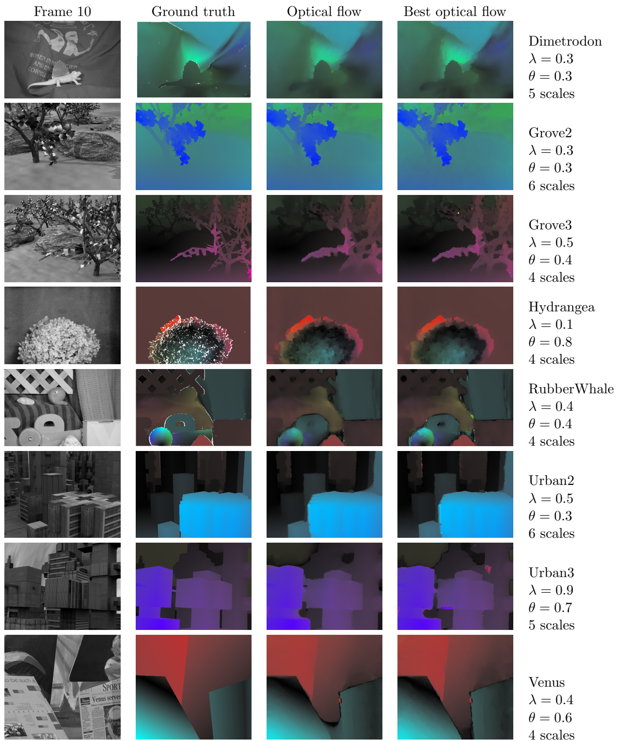
Figure 7: Results for the Middlebury test sequences.
