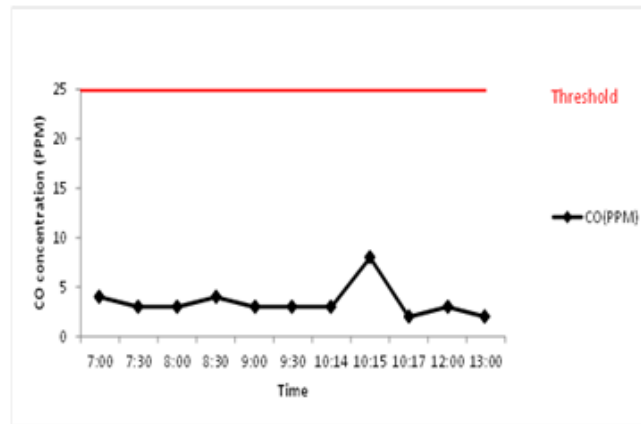
Fig. 8. CO concentration in the second experiment.
