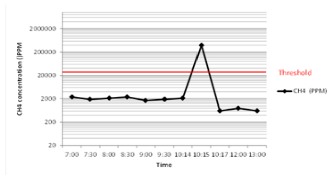
Fig. 7. CH4 concentration.
