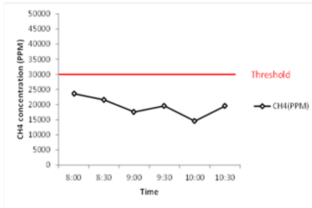
Fig. 6. CH4 concentration.
