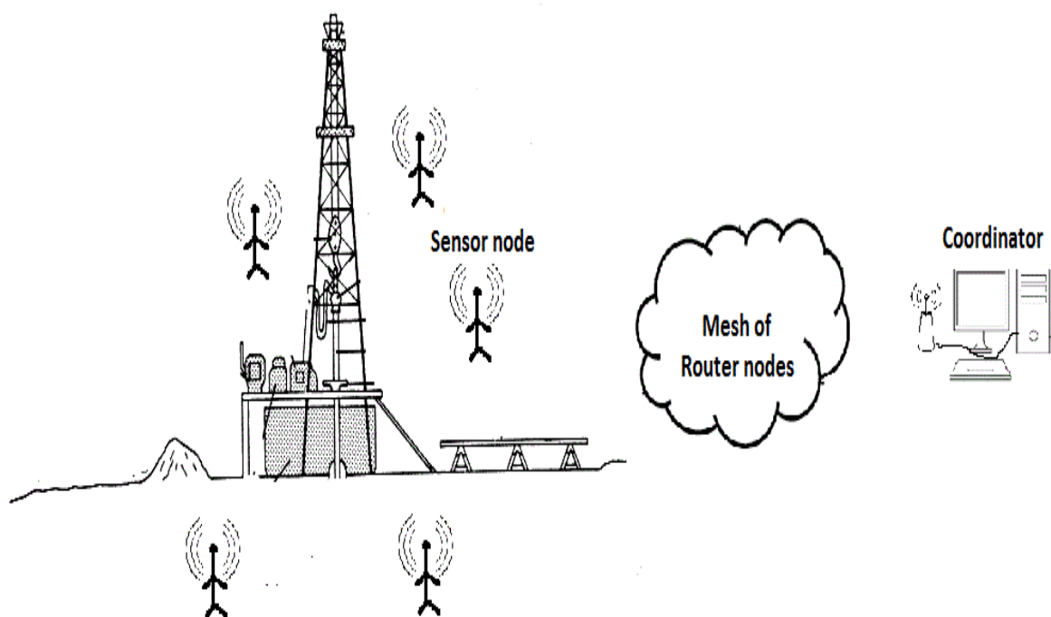
Fig. 1. System architecture.
