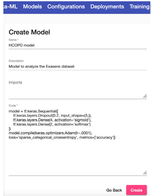
Fig. 8. Definition of the HCOPD ML model in Kafka-ML.
