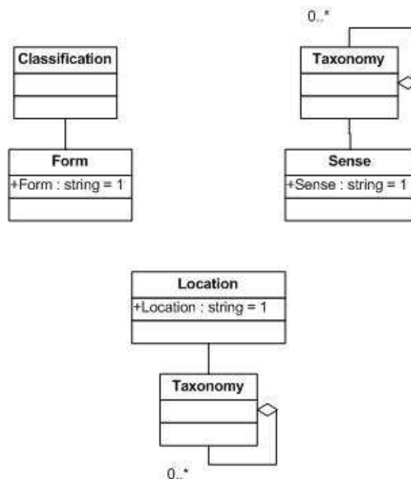
Figure 5: Core data types with classifications
