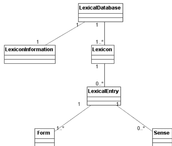
Figure 7: UML class diagram of LMF core model
