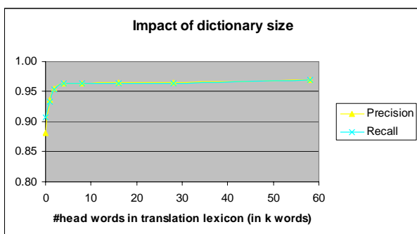
Figure 1: Precision and recall by dictionary size
