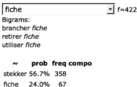
Figure 4: Querying bigrams
