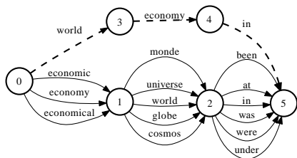
Figure 2: An example of lattice extension. The English phrase “world economy in” is appended to the lattice to change the word order.
