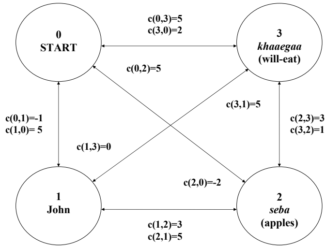
Figure 1: Example of an ATSP for reordering “John seba khaaegaa”
