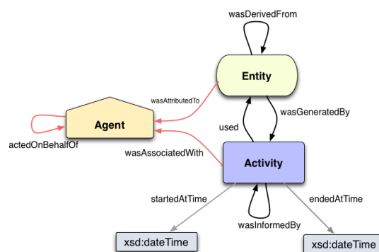
Figure 2: The PROV-DM
