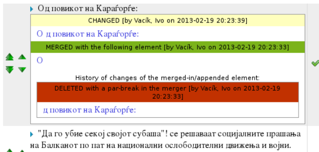
Figure 3: InterText server – editor interface detail showing the history of changes of one element in a Macedonian text.
