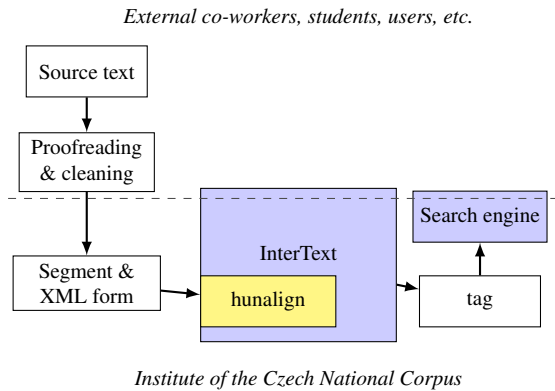
Figure 1: The task of InterText server in the current workflow in the InterCorp project.
