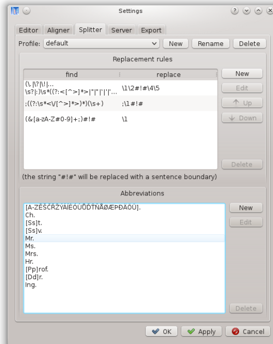
Figure 6: Sentence splitter can have several profiles configured as sets of replacement rules based on regular expressions and exceptions (“abbreviations”).
