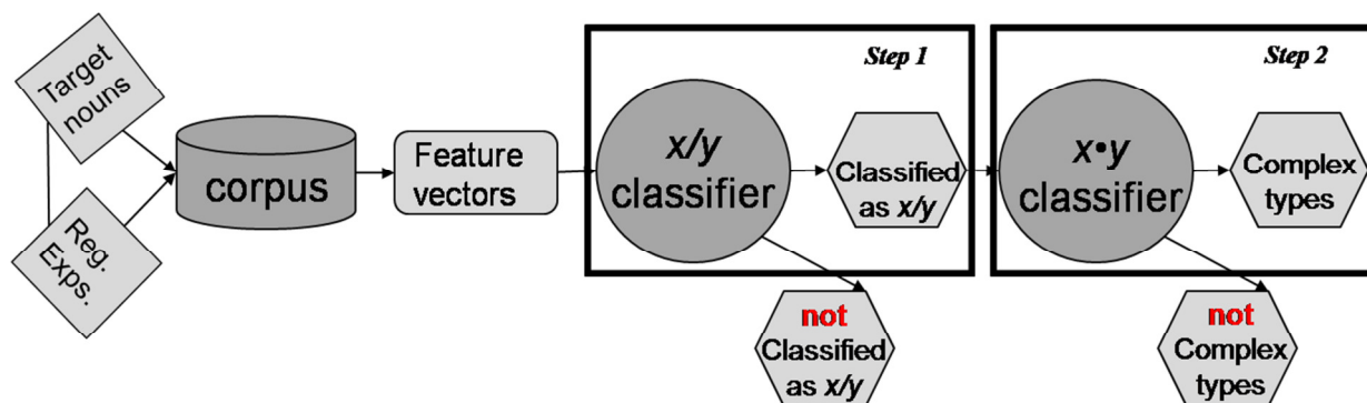
Figure 1: Workflow of the cascade experiment conducted for complex-type classification when no prior knowledge on the semantics of the nouns to be classified is available
