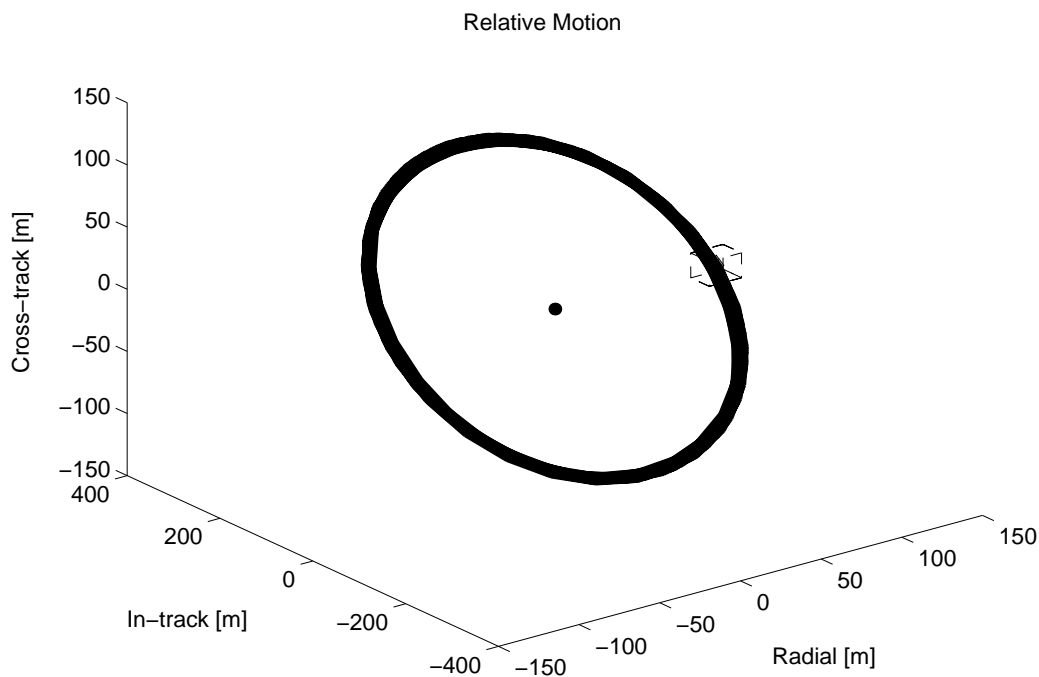
Figure 4-27: Relative motion of spacecraft during the two week simulation. The circle represents the formation center and the diamond enclosed in the box represents an example of the desired state and error box.
