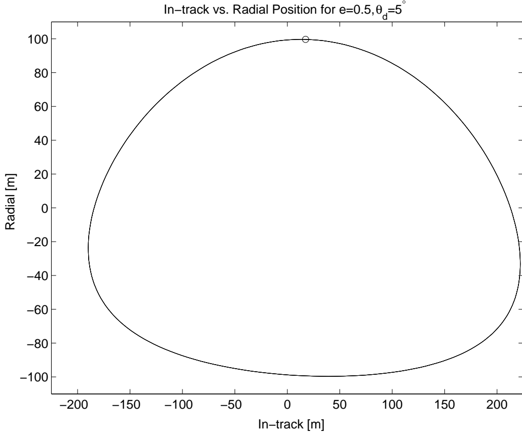
Figure 2-3: Trajectory followed for 4 orbits using initialization at \theta_d = 5^\circ . The \circ represents the initial constrained position. The periodic motion is now shifted off center and is not an ellipse.
