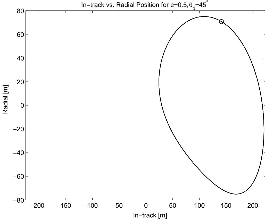
Figure 2-4: Trajectory followed for 4 orbits using initialization at \theta_d = 45^\circ . The \circ represents the initial constrained position. The periodic motion is clearly not centered about the origin.
