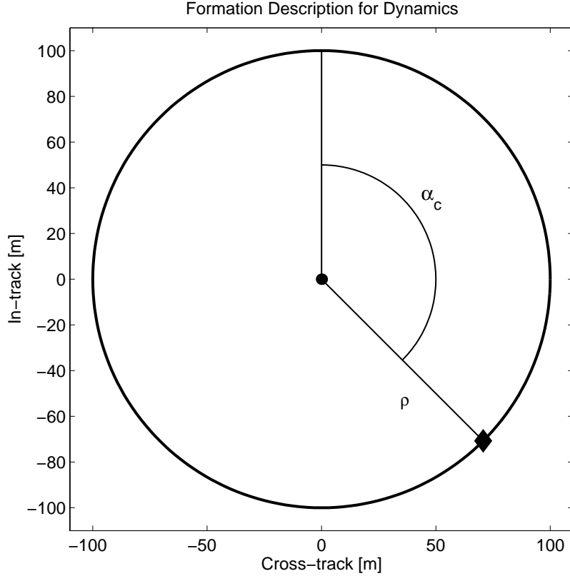
Figure 2-2: Typical formation description for a passive aperture that projects a circle in the in-track–cross-track plane. The cross-track phasing angle is measured by \alpha_c and \rho is the formation radius.
