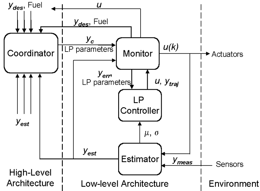
Figure 5-1: Low-level control diagram.
