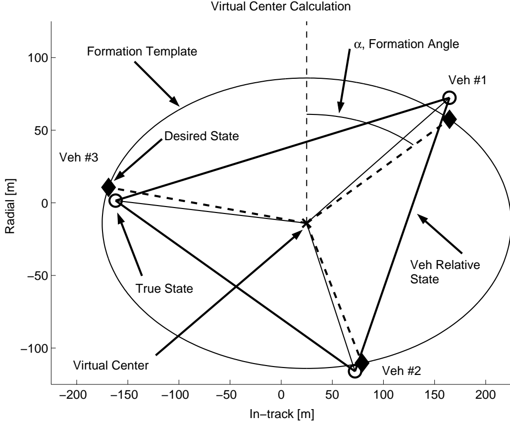
Figure 3-8: The virtual center can be calculated from the measured relative states (thick solid lines) and then used to determine the desired states (dashed lines) and actual state (thin solid lines) of each spacecraft relative to the center.
