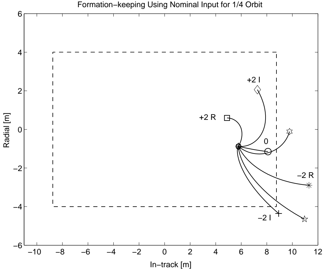
Figure 4-4: Trajectories for each of the five possible initial conditions using the plan for nominal case. The pentagram and hexagram represent two additional cases within the uncertainty ellipsoid but not considered in the plan.
