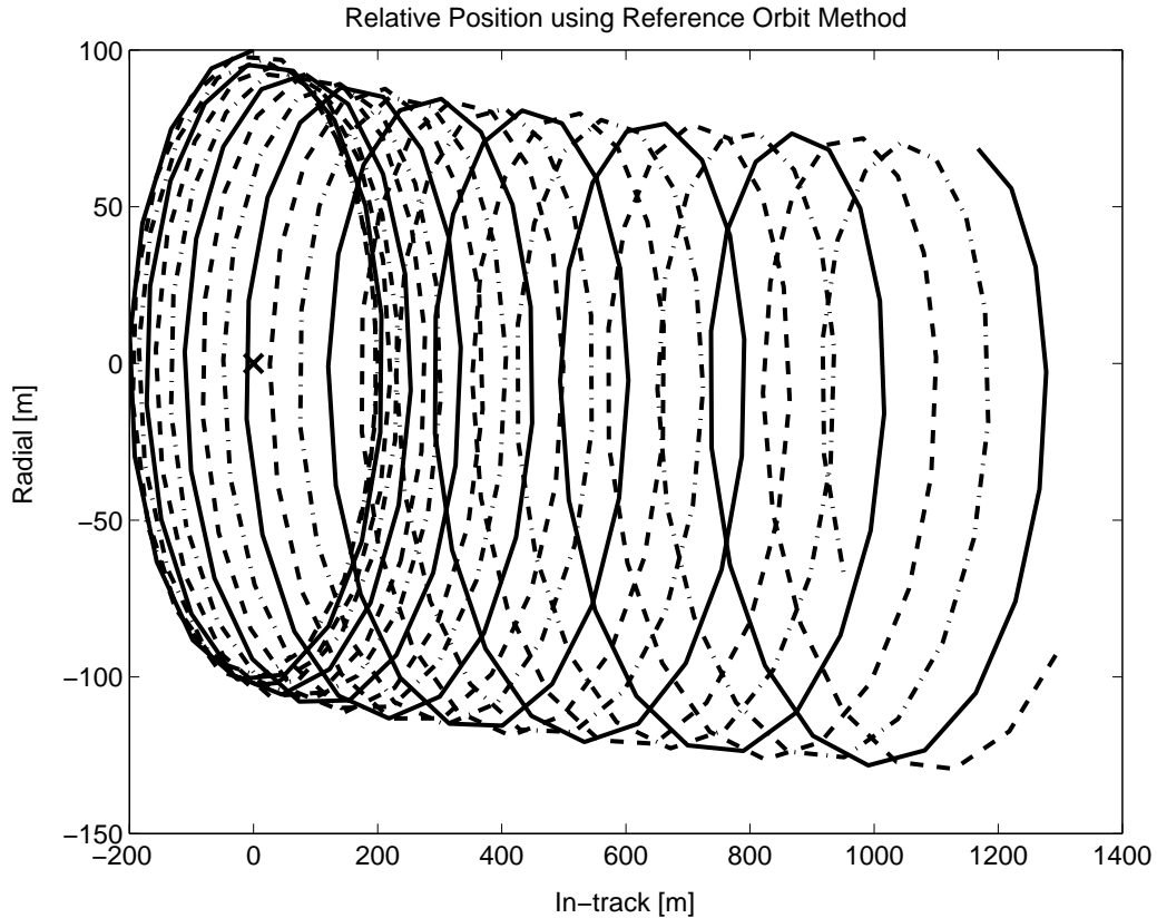
Figure 3-9: Relative motion with a reference point described by a reference orbit where the drag is modeled incorrectly. All the spacecraft drift from the aperture in the same direction due to a drag disturbance. The \times marks the reference point which is also the formation center.
