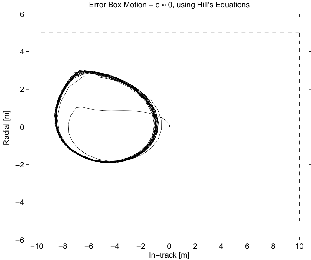
Figure 4-18: Error box motion for a reference orbit with e \approx 0 , using Hill's equations. The average fuel cost was 6.548 mm/s/orbit.
