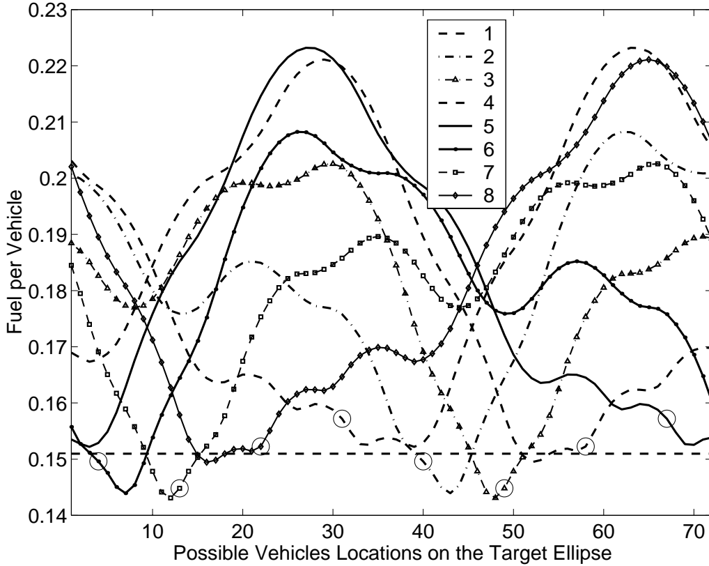
Figure 3-4: Associated predictions of the \Delta V fuel cost to move to each location on the target aperture. Uses a 5^\circ discretization of the target ellipse.
