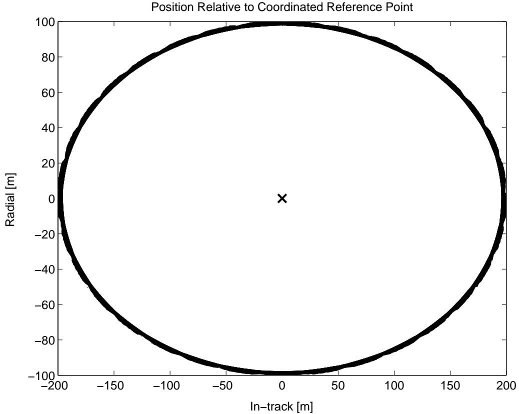
Figure 3-10: Relative motion with a reference point calculated using the virtual center method. The virtual center moves with the fleet resulting in no net disturbance force and the aperture is maintained. The \times marks the center.
