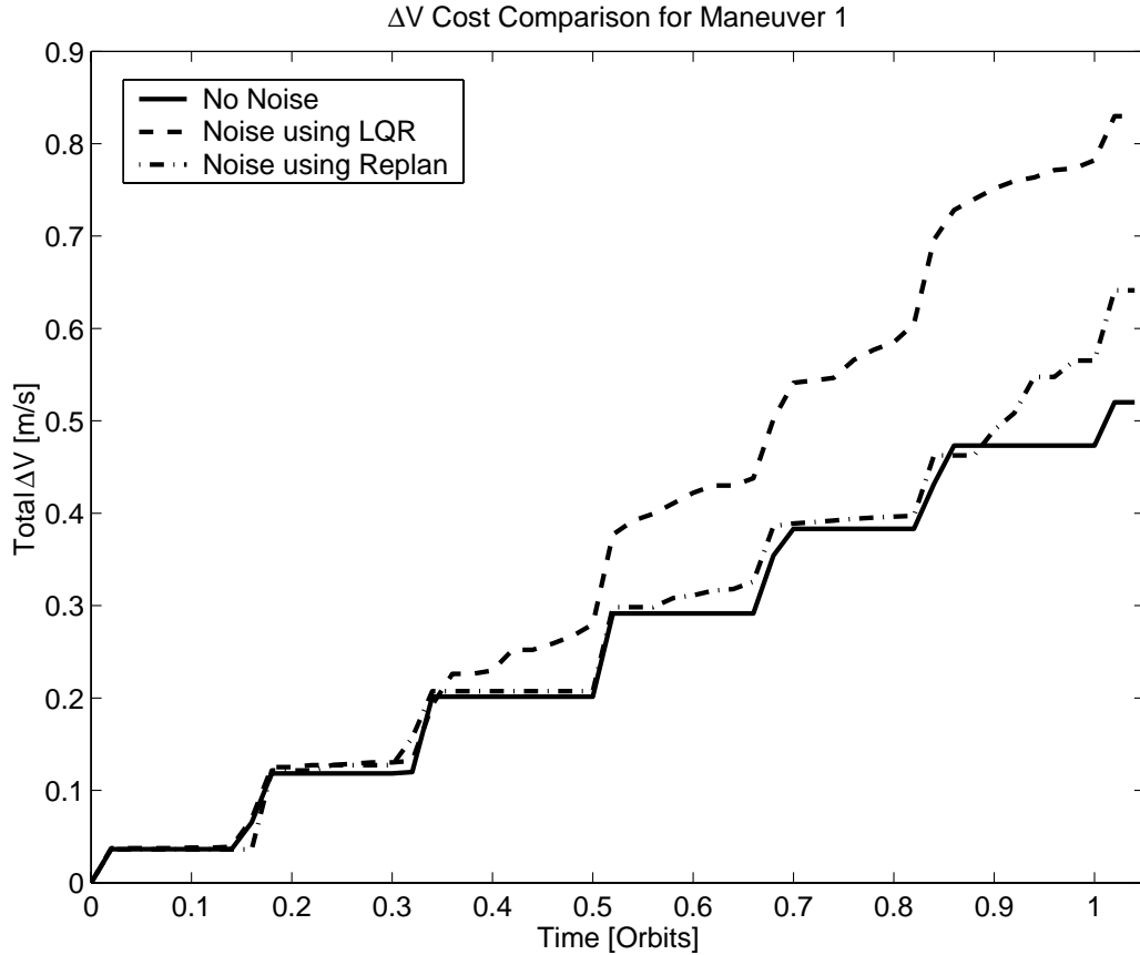
Figure 4-14: Total fuel ( \Delta V ) comparison using feed-forward, feed-forward/feedback LQR, and re-planning for the initialization maneuver. Total change in \Delta V = 0.310 m/s for feedback LQR and \Delta V = 0.121 m/s for re-planning.
