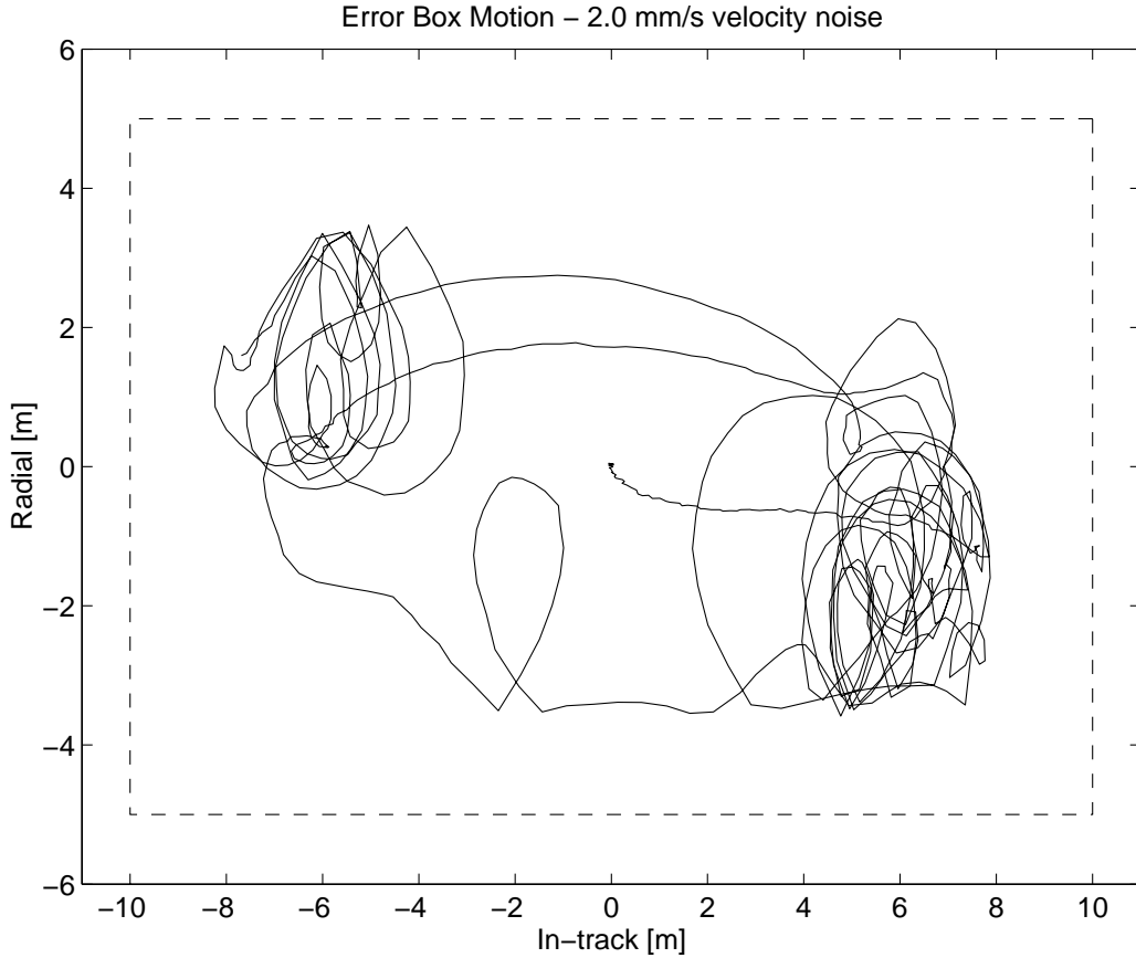
Figure 4-8: Typical motion for 2 mm/s velocity noise level.
