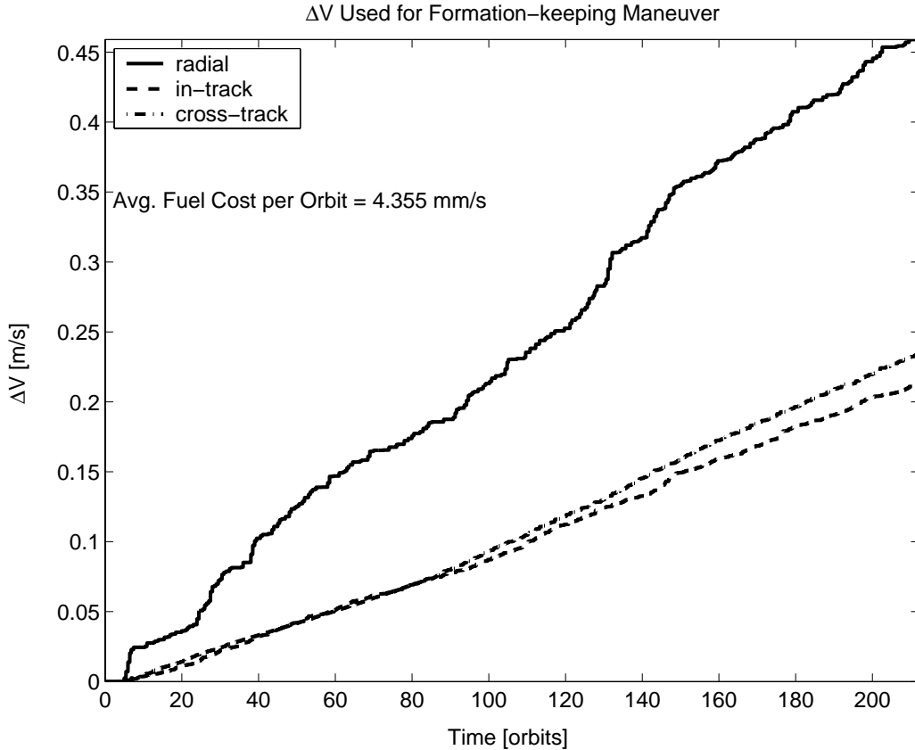
Figure 4-30: \Delta V fuel cost during simulation.
