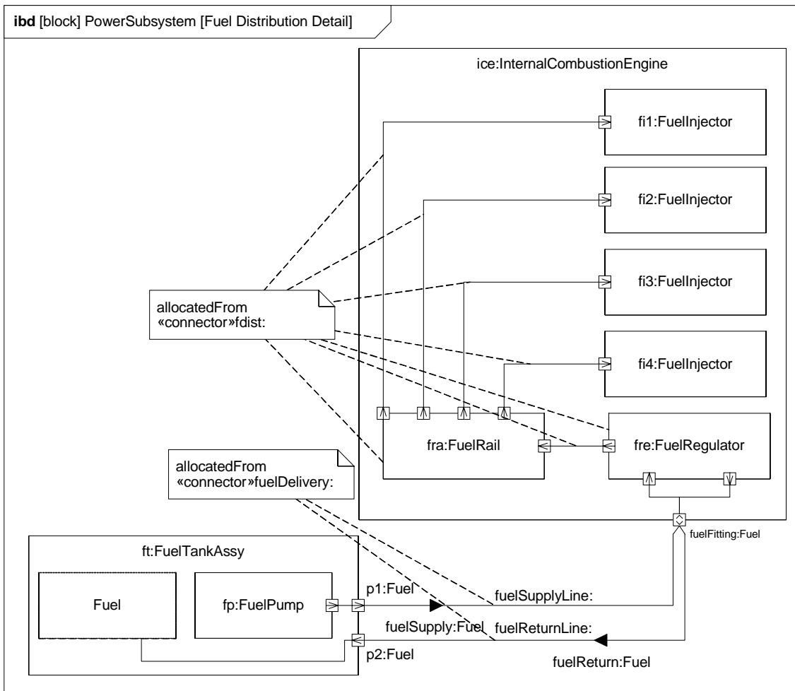
Figure 9.5 - Usage of atomic flow ports in the HybridSUV Sample - ibd:FuelDist diagram
