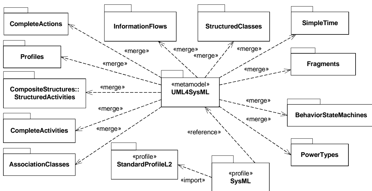
Figure 4.2 - SysML Extension of UML
