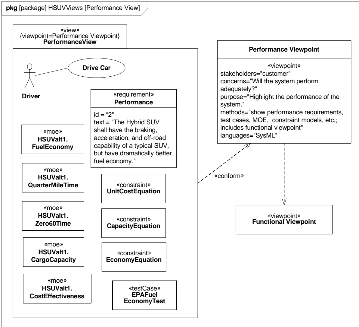
Figure 7.3 - View/Viewpoint example
