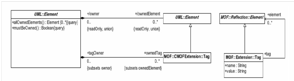
Figure 14.3 - CMOF Extension Package
