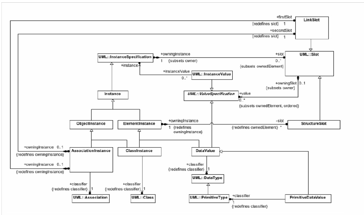
Figure 15.1 - Semantic Domain model for Constructs
