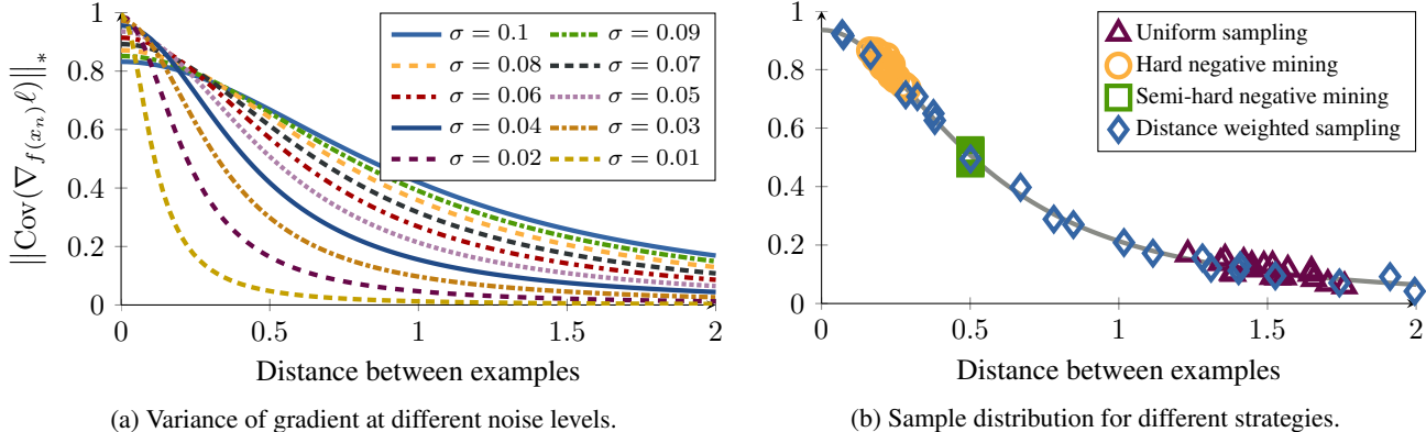
Figure 3: (a) shows the nuclear norm of a noisy gradient estimate for various levels of noise. High variance means the gradient is close to random, while low variance implies a deterministic gradient estimate. Lower is better. Note that higher noise levels have a lower variance at distance 0. This is due to the spherical projection imposed by the normalization. (b) shows the empirical distribution of samples drawn for different strategies. Distance weighted sampling selects a wide range of samples, while all other approaches are biased towards certain distances.
