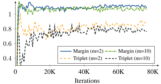
Figure 6: Optimal validation threshold for the LFW dataset. Triplet loss with different sampling strategies converges to different solutions. In addition, it has large fluctuations in the early stage, indicating unstable training. Margin based loss always converges stably to the same solution.
