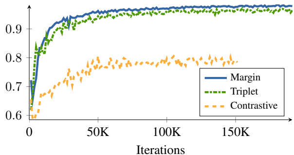
Figure 7: Validation accuracy curve, trained on CASIA-WebFace and evaluated on LFW. The margin based loss with distance weighted sampling converges quickly and stably, outperforming other methods.
