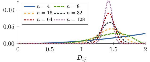
Figure 2: Density of datapoints on the D -dimensional unit sphere. Note the concentration of measure as the dimensionality increases — most points are almost equidistant.
