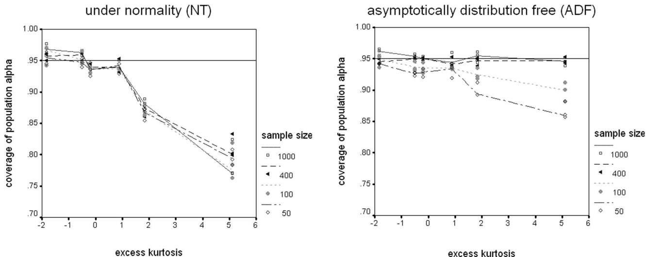
Figure 7. Proportion of times (coverage) that 95% confidence intervals (CIs) for coefficient alpha include population coefficient alpha as a function of kurtosis and sample size. Data have been generated according to a congeneric model. Coverage rates should be close to nominal rates (95%). A nonparametric procedure has been used to model the relationship between coverage and excess kurtosis by sample size. The accuracy of both CIs is similar (and adequate) for items with low excess kurtosis (< 1). For items with higher excess kurtosis, asymptotically distribution-free (ADF) intervals are more accurate, particularly when sample size is greater than 100 observations.
