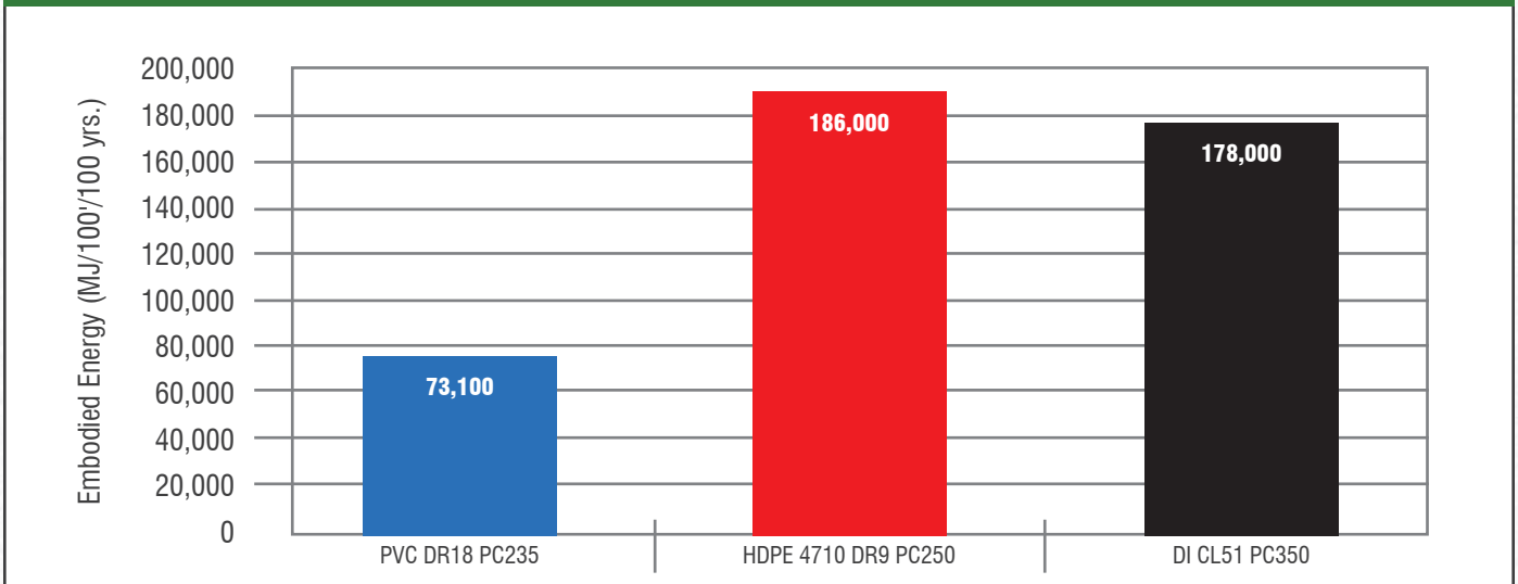
FIGURE A.5 : 8" PVC DR18 EQUIVALENT PIPES: 100-YEAR TOTAL EMBODIED ENERGY
