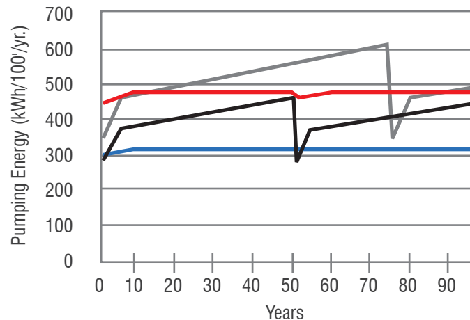
FIGURE 8.4 : ANNUAL PUMPING ENERGY COMPARISONS FOR 24" PIPES
