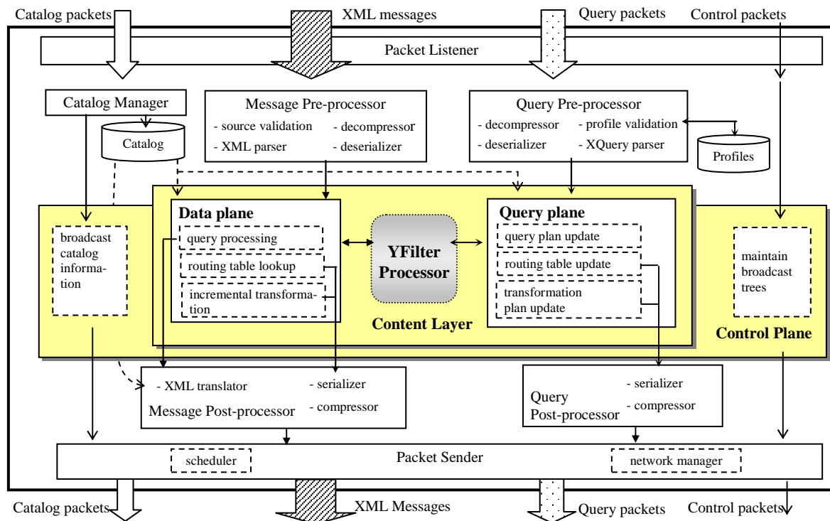
Fig. 10. Broker Architecture
