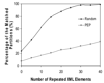
Fig. 9. Random query partitioning vs. PEP
