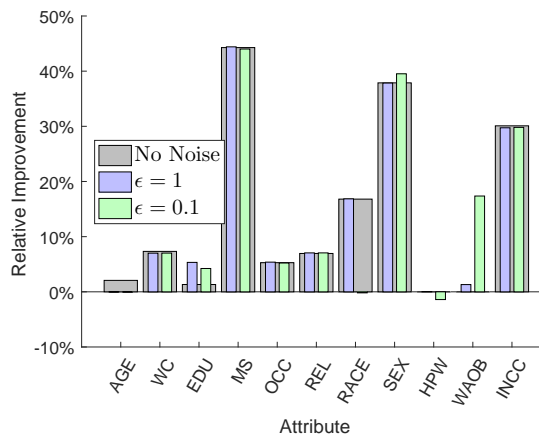
Figure 1: Relative Improvement of Model Accuracy of the un-noised, \epsilon = 1 -DP, and \epsilon = 0.1 -DP models, with respect to the baseline (marginals). Overall, the improvement for \epsilon = 1 or \epsilon = 0.1 is comparable to that for the un-noised version. Adding noise to achieve DP for structure learning (Section 3.3) can lead to a different acyclic graph of the model. (This is why there is a significant difference in improvement for attributes RACE and WAOB between \epsilon = 1 -DP and \epsilon = 0.1 -DP.)
