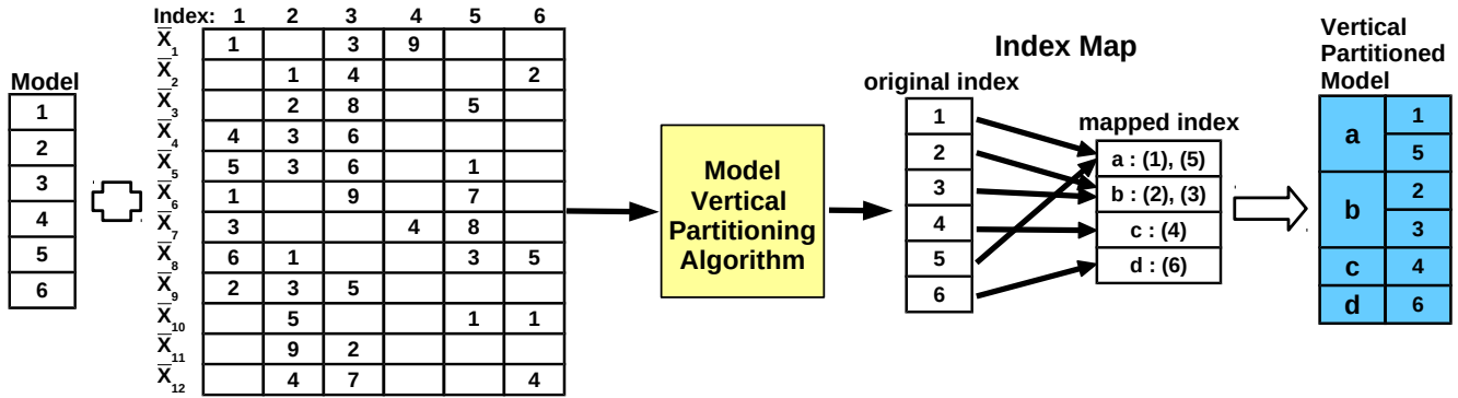
Figure 2: The offline model vertical partitioning stage.
