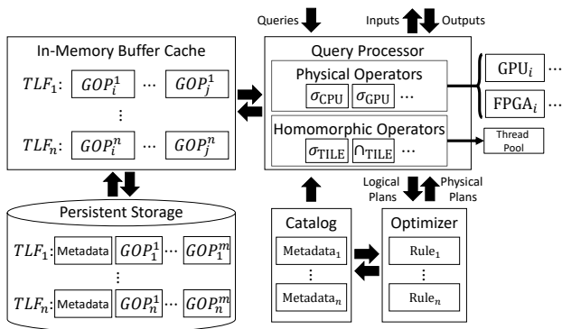
Figure 9: LightDB architecture
