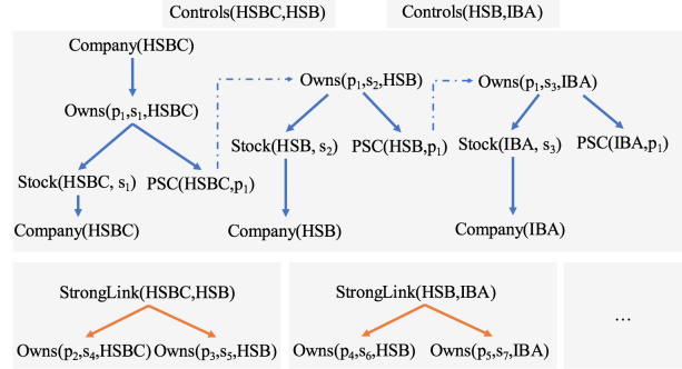
Figure 2: A portion of the warded forest for the chase graph of rules in Example 3. Solid edges denote linear rules and the dash-dotted edges denote joins in warded rules.
