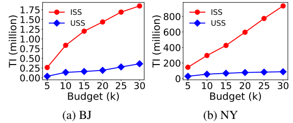
Figure 9: The total improvement (TI) on (a) BJ and (c) NY.
