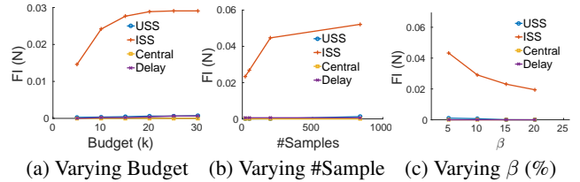
Figure 7: (NY) The flow improvement (FI) by varying (a) budget, (b) the number of samples, and (c) \beta (%).
