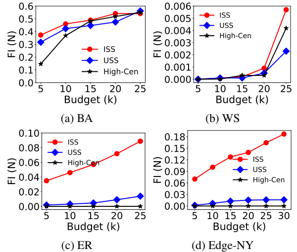
Figure 11: Comparison of Flow Improvement FI(N) between ISS and other baselines varying budget ( k ) (a-c) Synthetic Network Structure: on (a) BA, (b) WS, and (c) ER graph generation models; (d) when the delays are on the edges.
