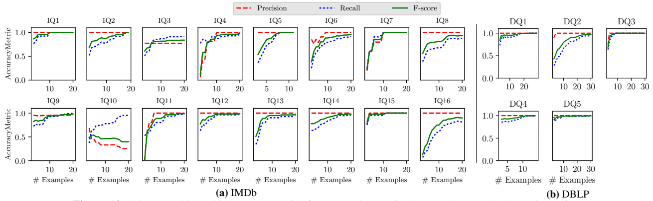
Figure 10: SQUID achieves high accuracy with few examples (typically \sim 5 ) in most benchmark queries.
