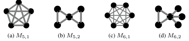
Figure 10: Motif Representatives
