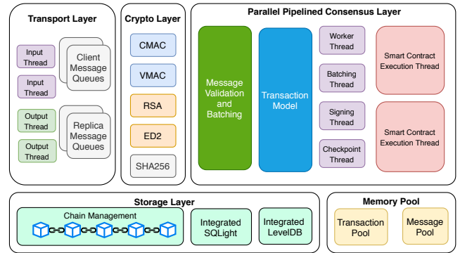
Figure 2: Architecture of the ResilientDB fabric.
