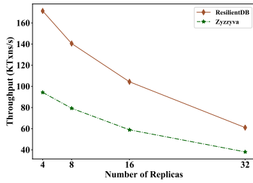
Figure 1: Two permissioned applications employing distinct Bft protocols (80k clients per experiment).
