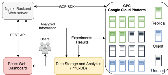
Figure 3: Demo Platform Architecture.
