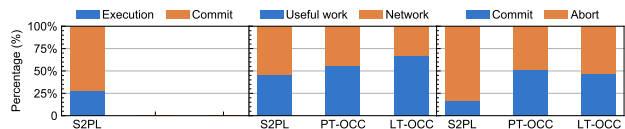
Figure 14: Breakdown on TPC-C in a wide-area network
