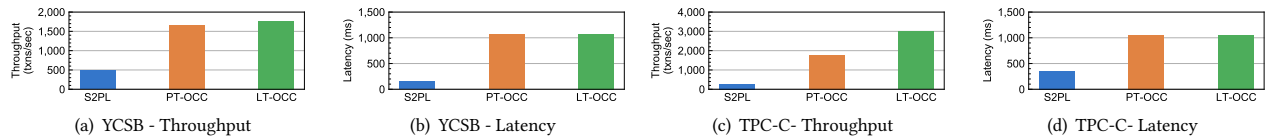
Figure 12: Performance of 2PC(Sync) and Epoch(Async) in a wide-area network
