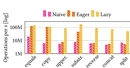
Figure 12: Text processing.
