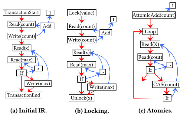
Figure 6: Operator-IR of stateful UDF.
