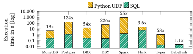
Figure 1: Overhead of TPC-H Query 6 with Python UDF.
